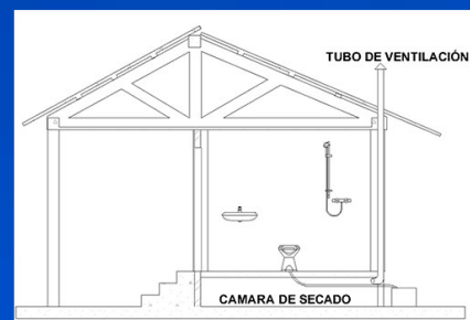
TOILET DESIGN
