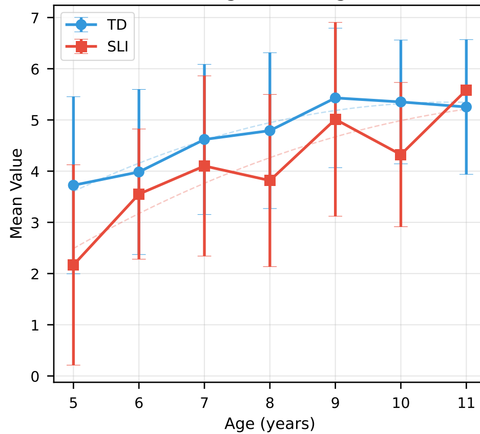
Transitivity
