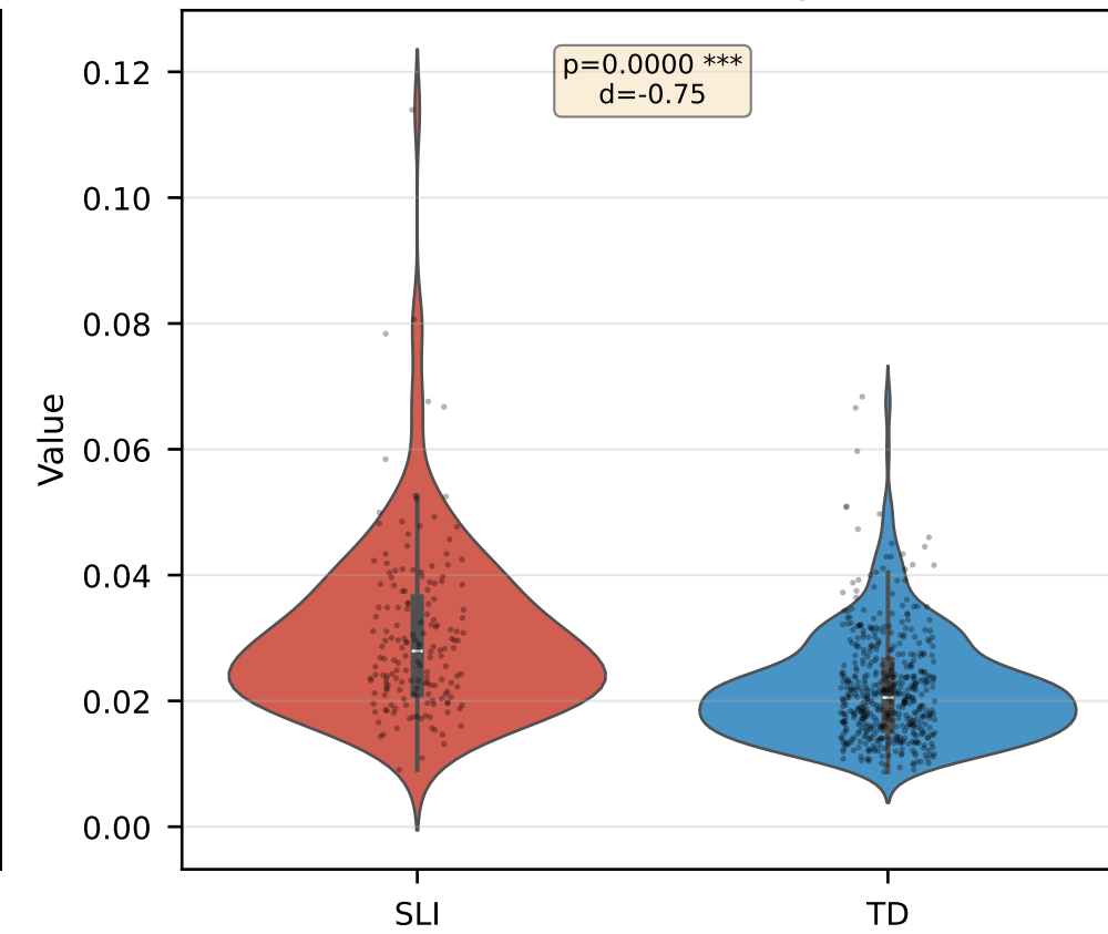
Network Density
