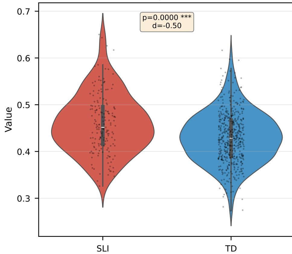
Degree Centrality
