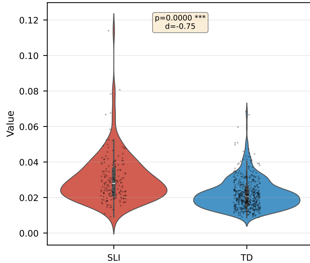
Degree Centrality
