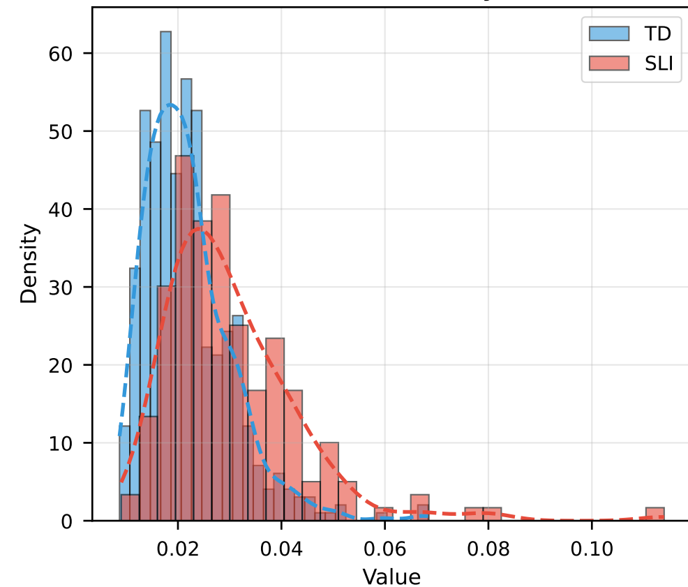
Network Density
