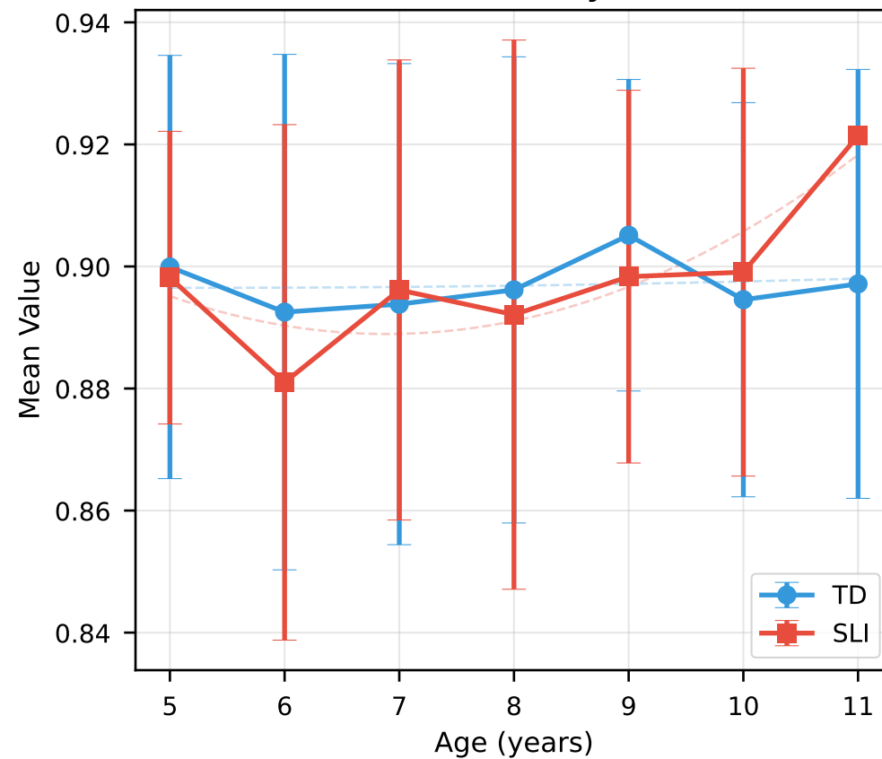
Transitivity
