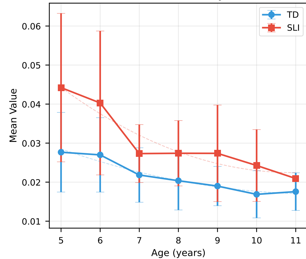
Network Density
