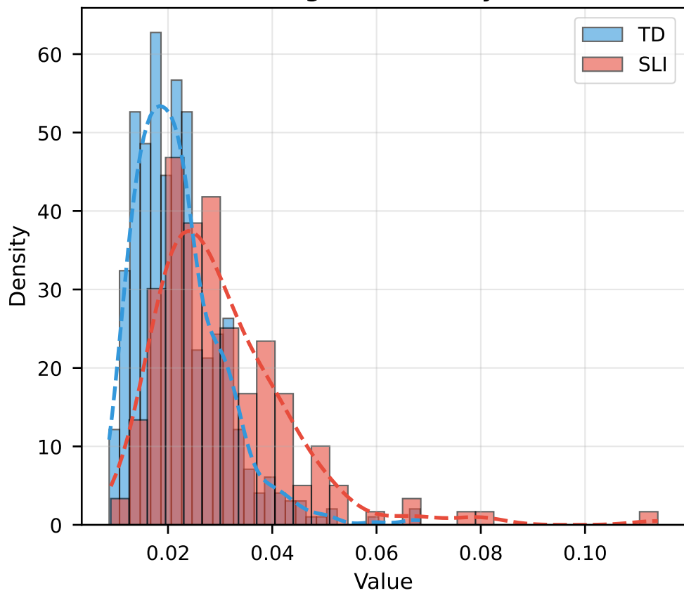
Degree Centrality
