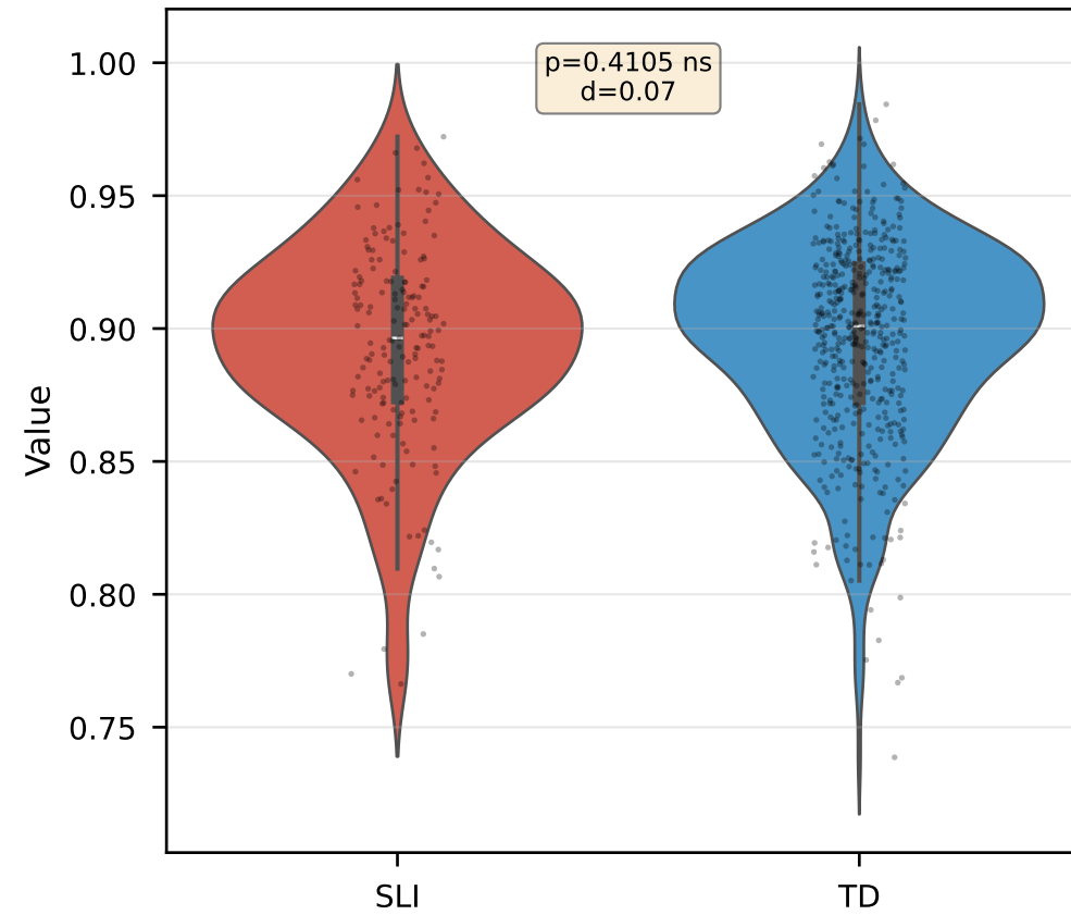
Transitivity
