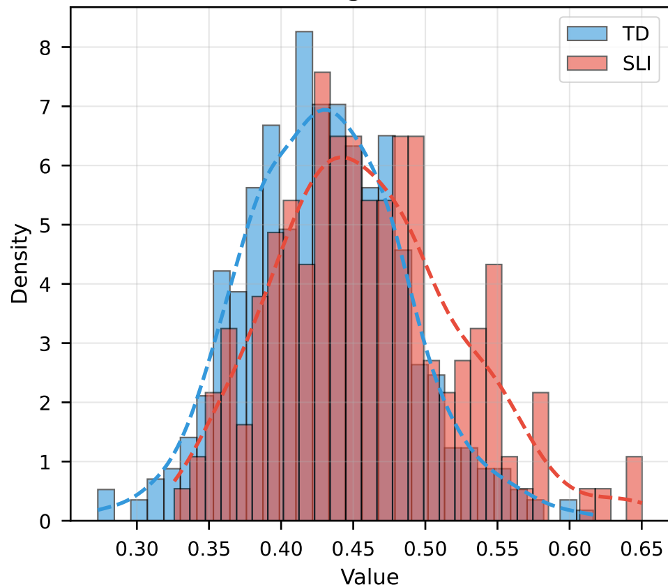
Clustering Coefficient
