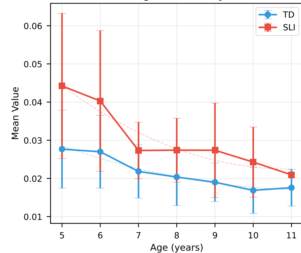
Degree Centrality
