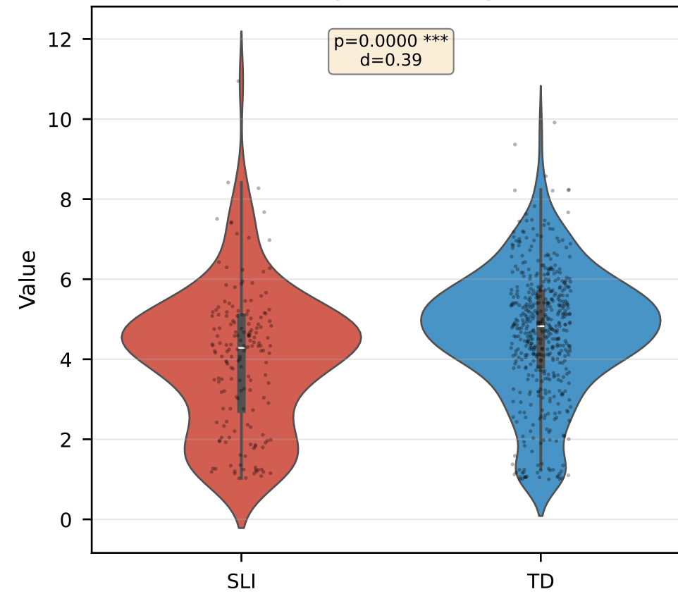
Transitivity
