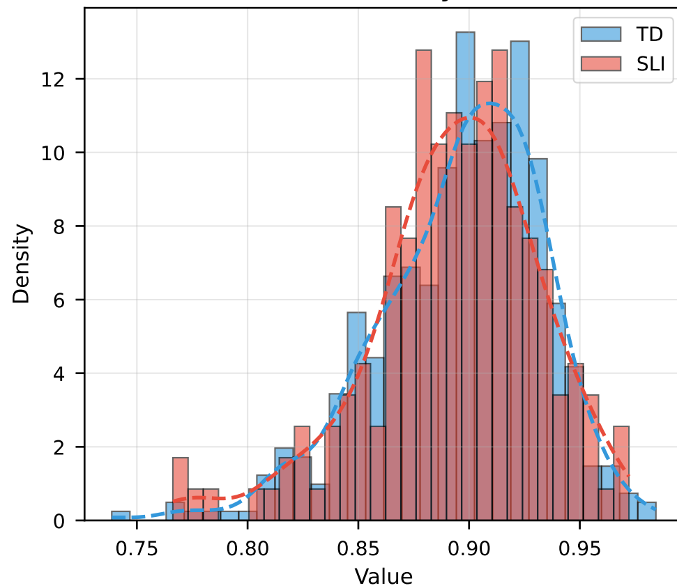
Transitivity
