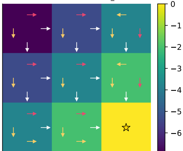
Value Iteration — fixture_3x3
