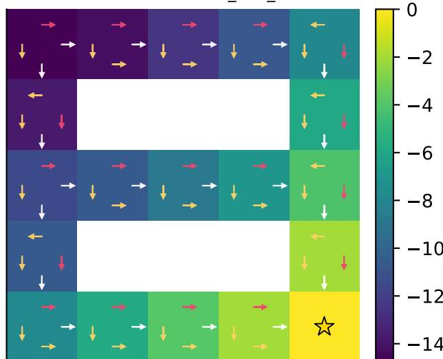
Value Iteration — fixture_5x5_corridor
