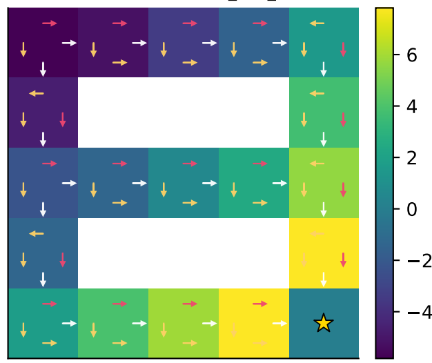
SARSA — fixture_5x5_corridor
