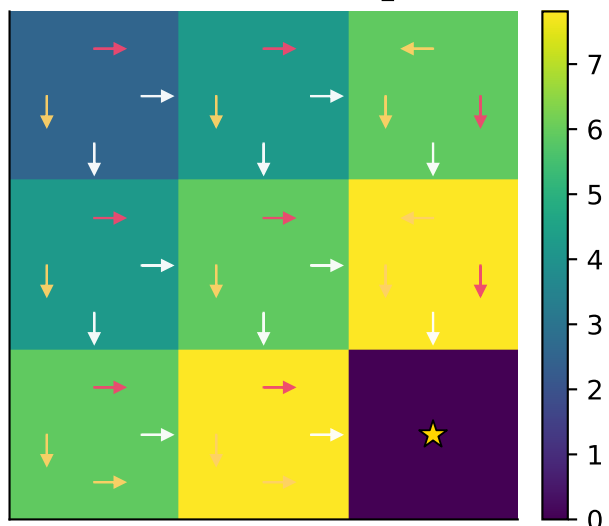
SARSA — fixture_3x3
