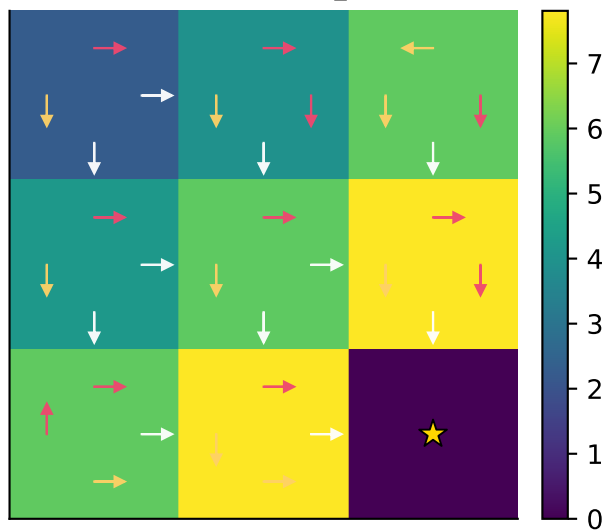
Q-Learning — fixture_3x3
