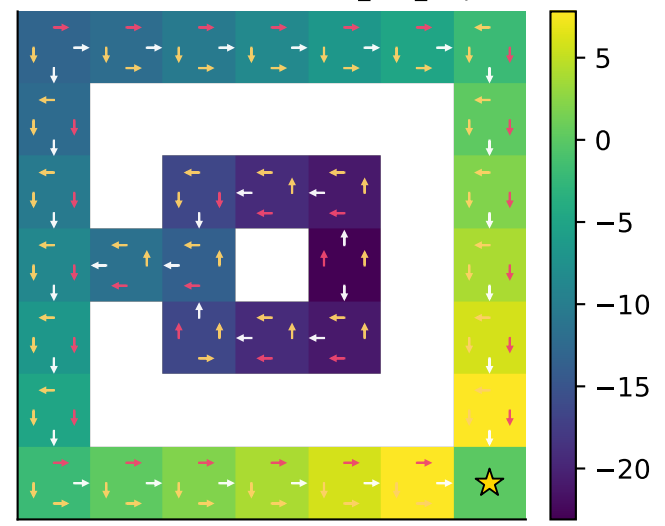
SARSA — fixture_7x7_loop
