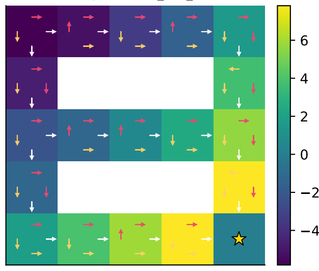
Q-Learning — fixture_5x5_corridor
