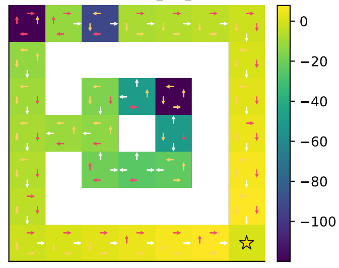
Q-Learning — fixture_7x7_loop
