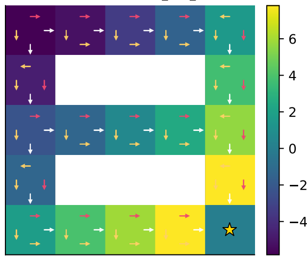
Value Iteration — fixture_5x5_corridor
