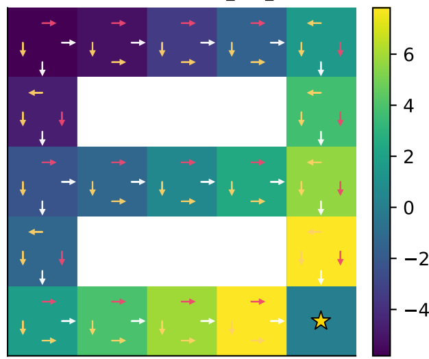
Value Iteration — fixture_5x5_corridor
