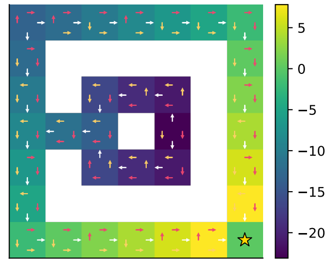
Q-Learning — fixture_7x7_loop
