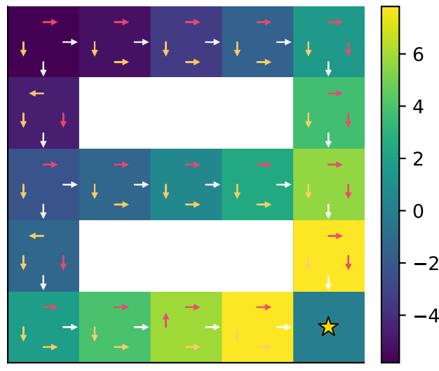
Q-Learning — fixture_5x5_corridor
