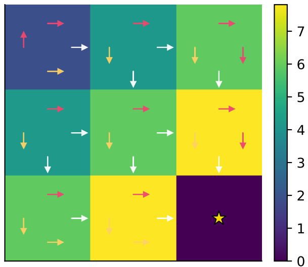
Q-Learning — fixture_3x3
