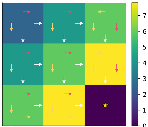
Value Iteration — fixture_3x3
