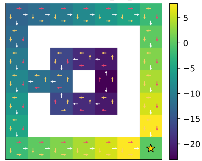
Value Iteration — fixture_7x7_loop
