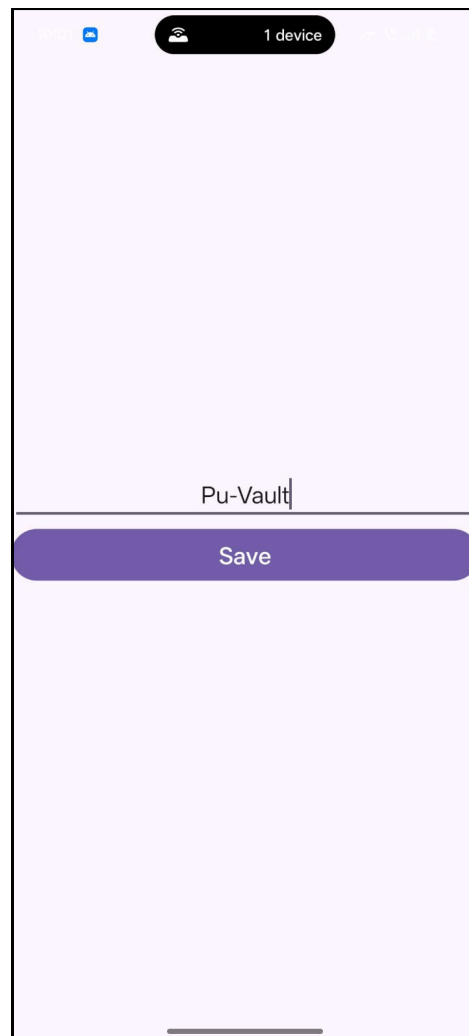
SavedInstanceState
