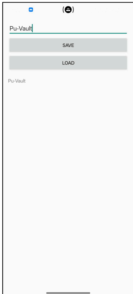
Shared Preference
