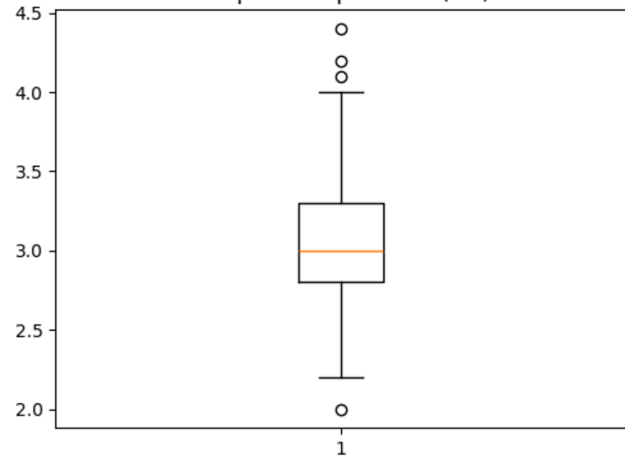
Box plot of sepal width (cm)
