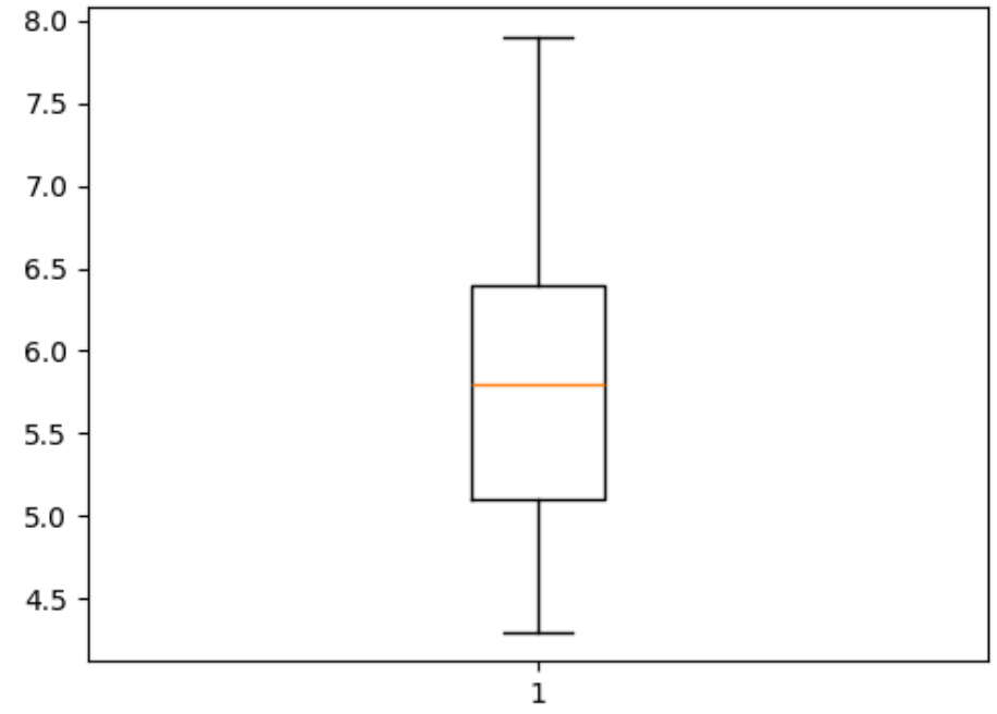
Box plot of sepal length (cm)
