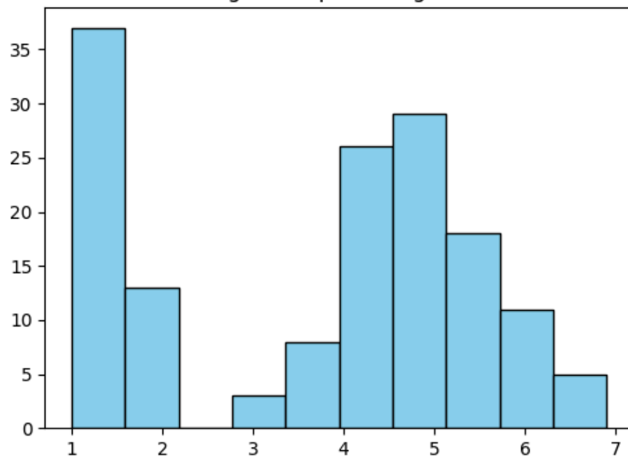
Histogram of petal length (cm)
