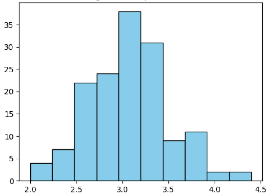
Histogram of sepal width (cm)
