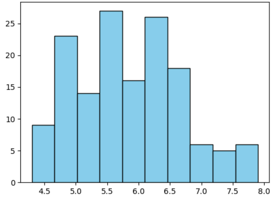
Histogram of sepal length (cm)
