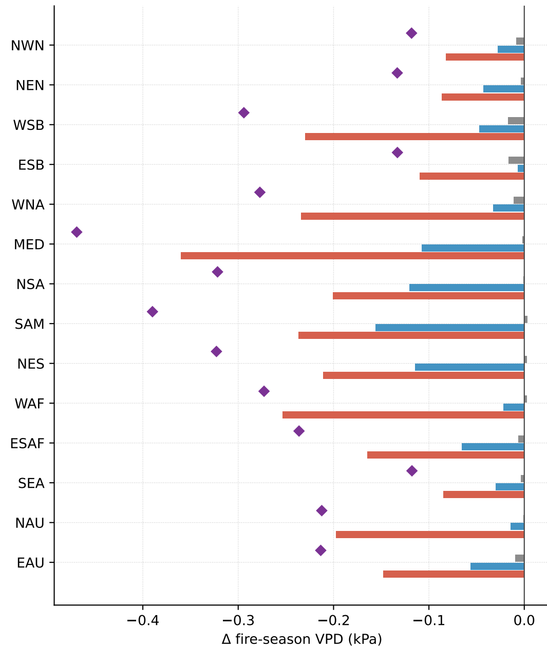
G6-1.5K-SAI – SSP2-4.5 (model mean)
