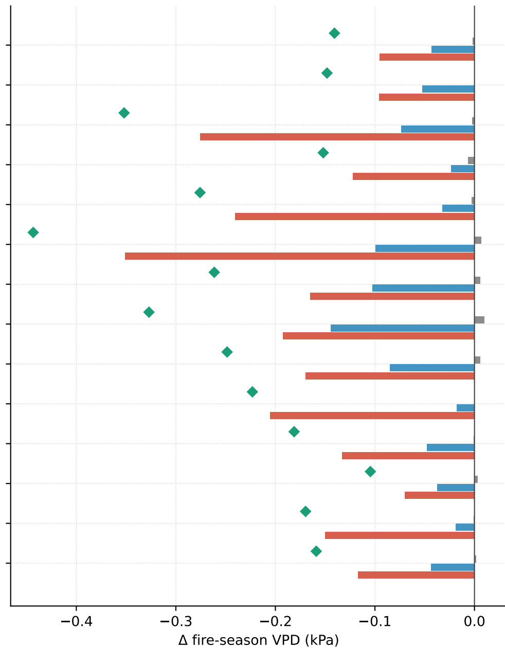
G6-1.5K-HiLLA – SSP2-4.5 (model mean)
