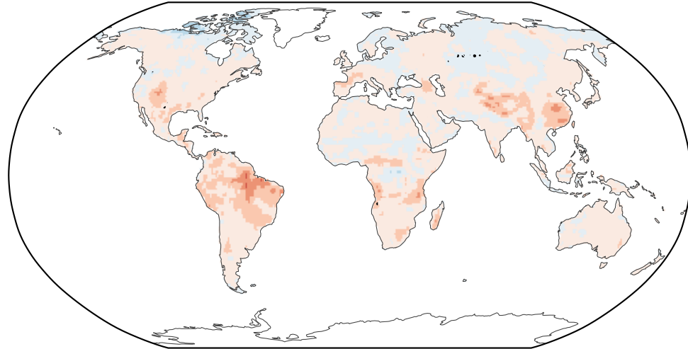
Multi-model mean G6-HiLLA – G6-SAI
