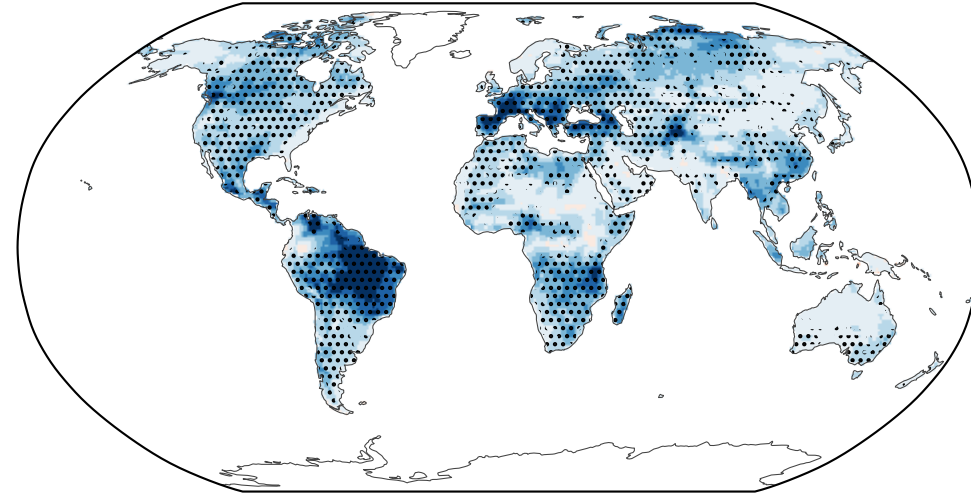
Multi-model mean G6-SAI – SSP2-4.5
