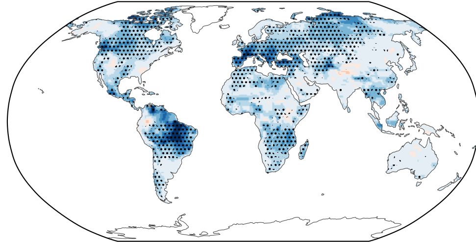
Multi-model mean G6-HiLLA – SSP2-4.5
