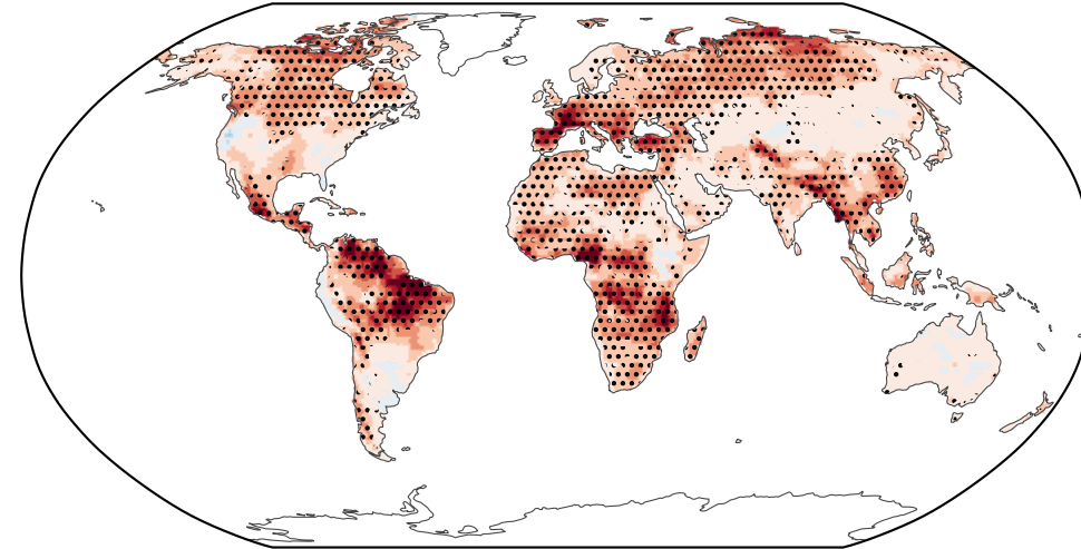
Multi-model mean SSP2-4.5 (2064-83) – target
