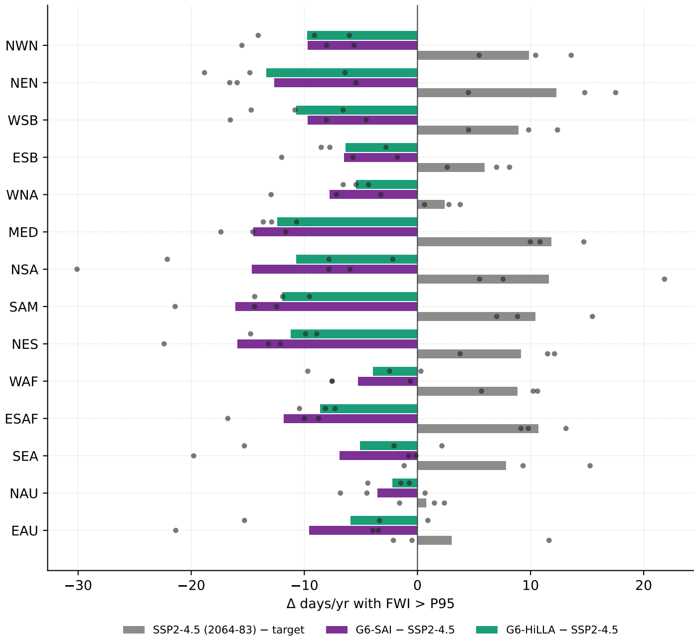
AR6 focus regions (CESM2-WACCM, MIROC-ES2H, UKESM1-1)
