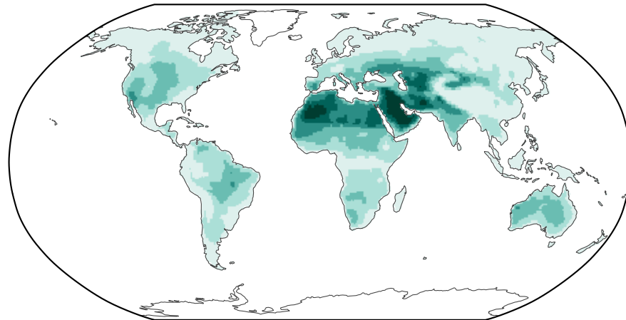
G6-1.5K-SAI – SSP2-4.5 Temperature term
