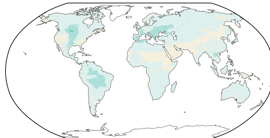
G6-1.5K-HiLLA – SSP2-4.5 Humidity (RH) term
