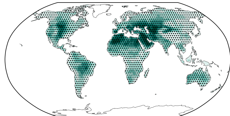
G6-1.5K-HiLLA – SSP2-4.5 \Delta VPD (total)
