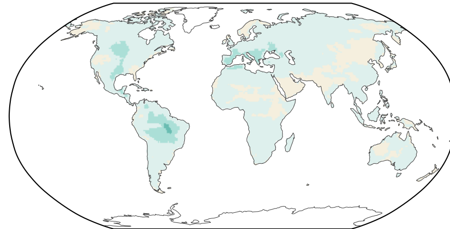
G6-1.5K-SAI – SSP2-4.5 Humidity (RH) term
