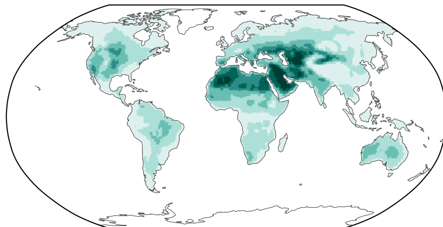
G6-1.5K-HiLLA – SSP2-4.5 Temperature term
