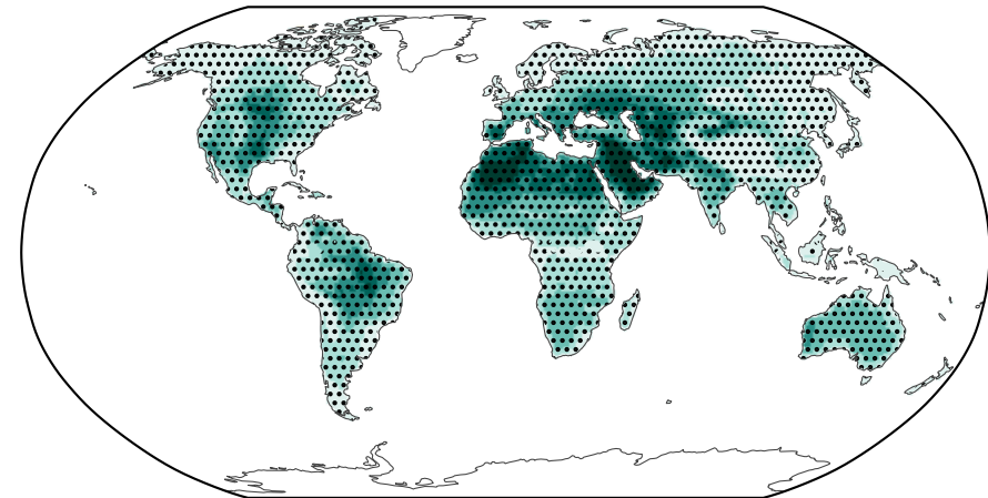
G6-1.5K-SAI – SSP2-4.5 \Delta VPD (total)
