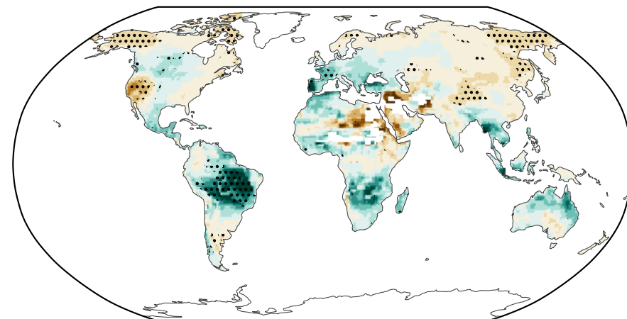
G6-1.5K-HiLLA – SSP2-4.5 \Delta precipitation
