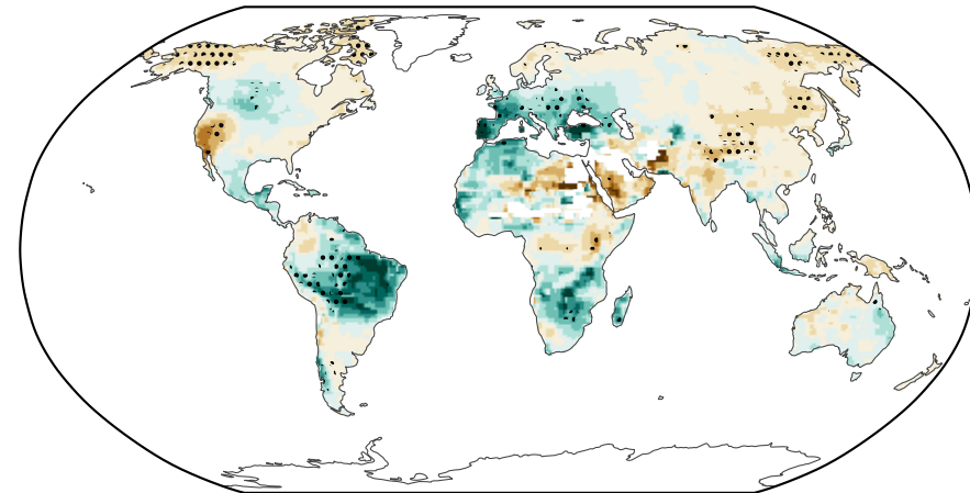
G6-1.5K-SAI – SSP2-4.5 \Delta precipitation
