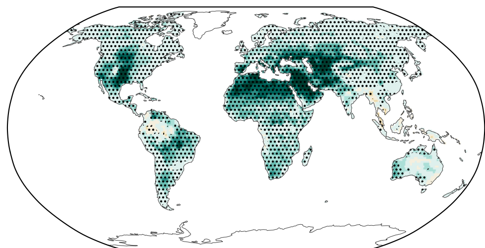
UKESM1-1 G6-HiLLA – SSP2-4.5
