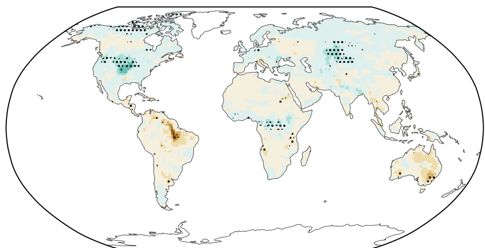
UKESM1-1 G6-HiLLA – G6-SAI
