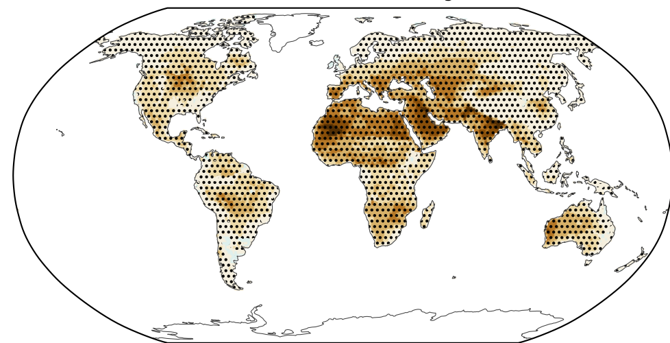
CESM2-WACCM SSP2-4.5 (2064-83) – target
