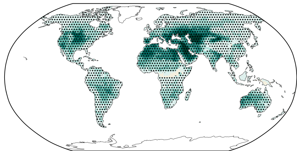
CESM2-WACCM G6-HiLLA – SSP2-4.5
