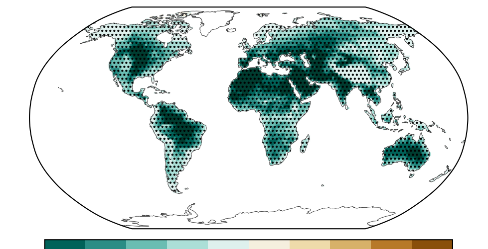
UKESM1-1 G6-SAI – SSP2-4.5
