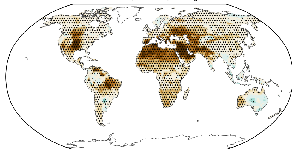
UKESM1-1 SSP2-4.5 (2064-83) – target
