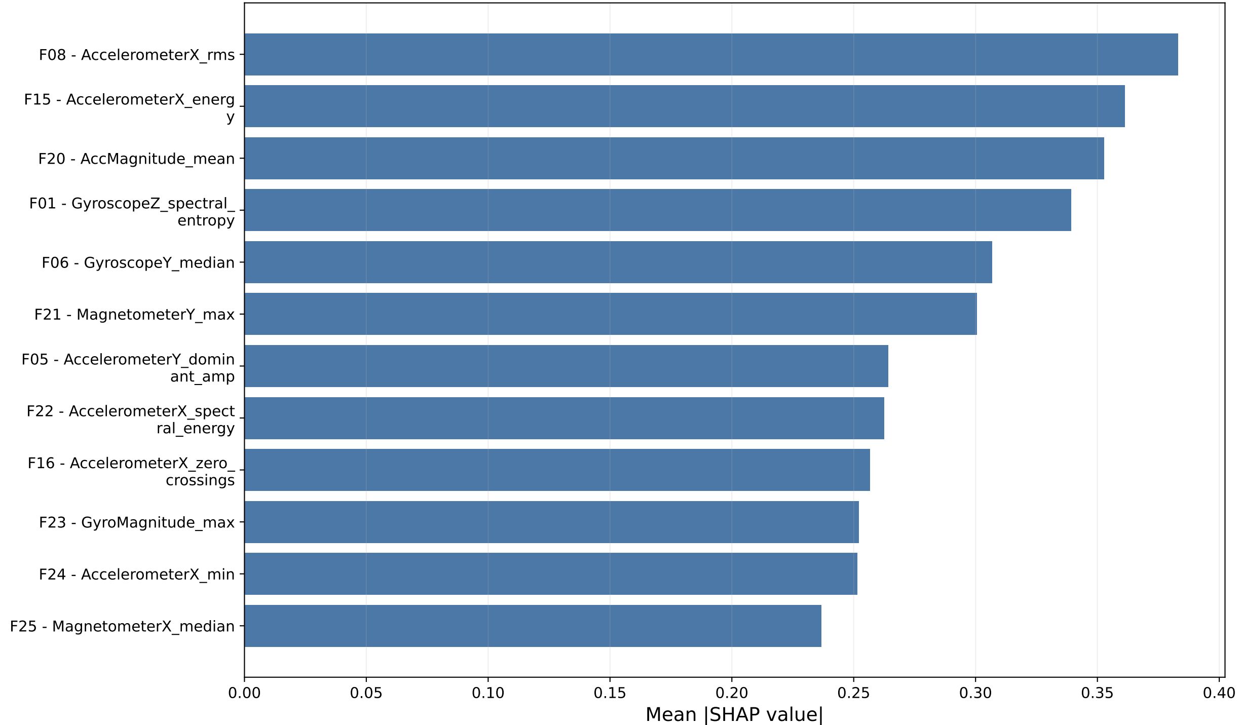
Logistic Regression (tuned): Top SHAP Features with Alias Labels
