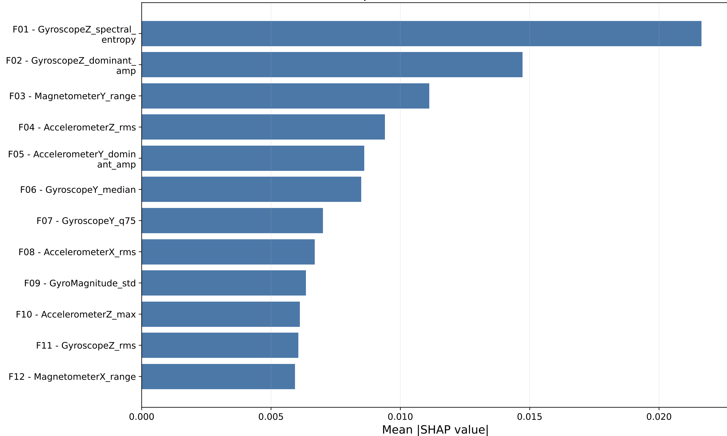
SVM (RBF): Top SHAP Features with Alias Labels
