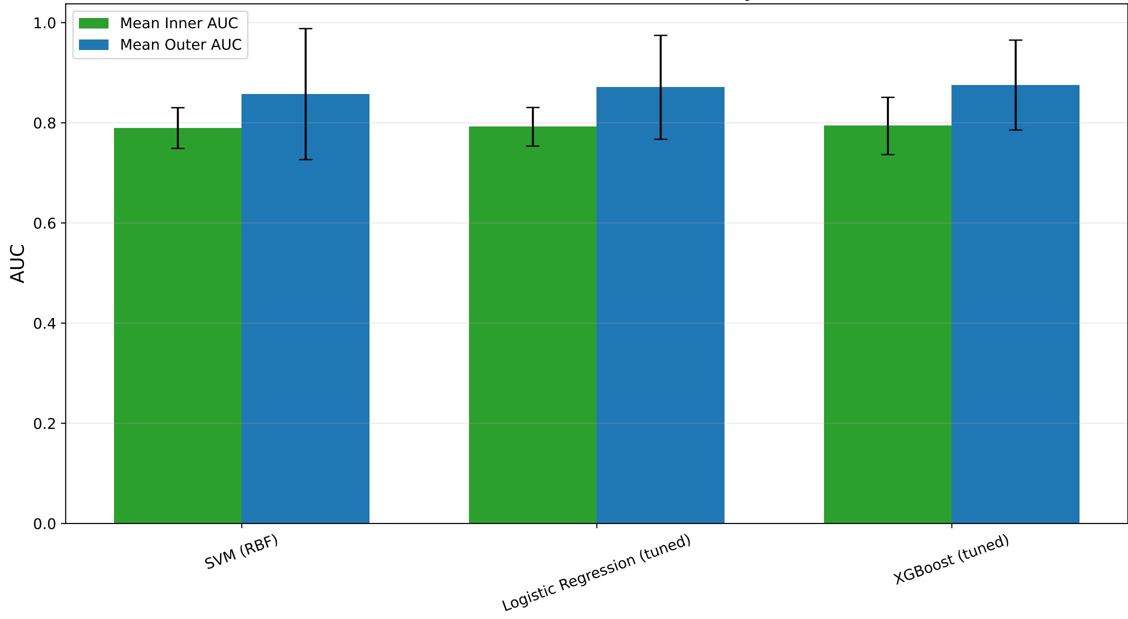
Mean Inner vs Outer AUC-ROC by Model
