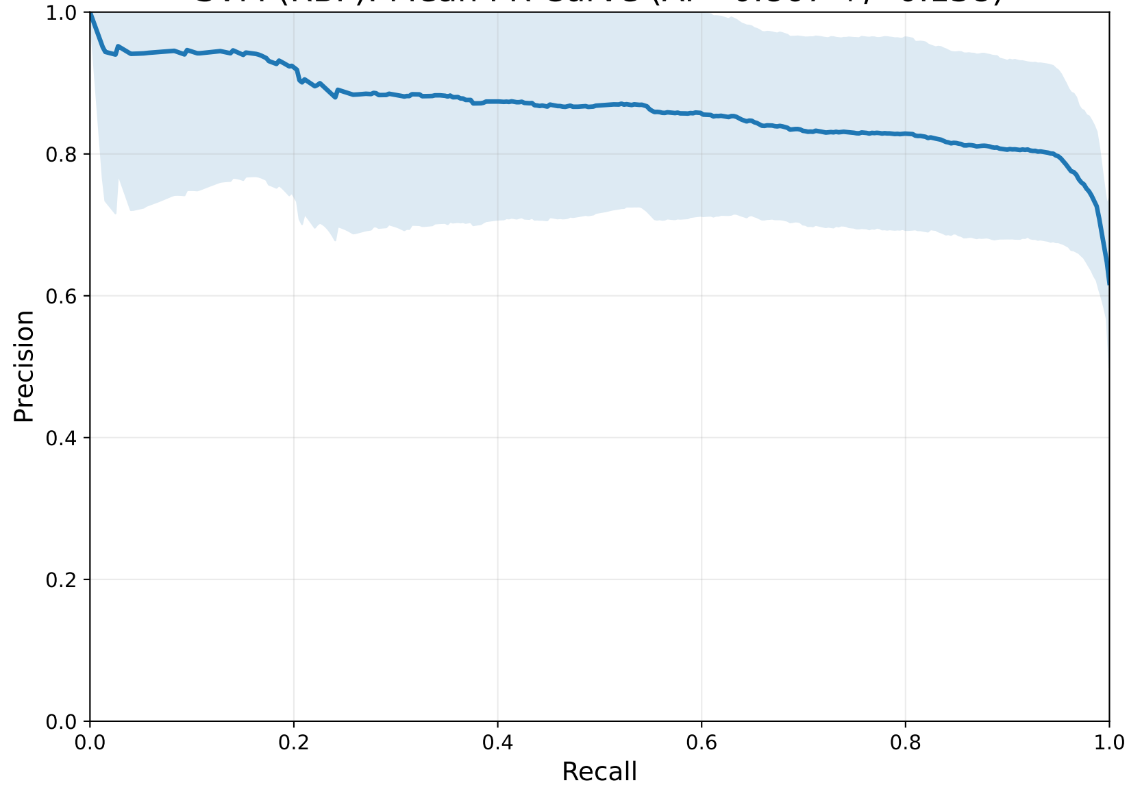
SVM (RBF): Mean PR Curve (AP=0.867 +/- 0.138)
