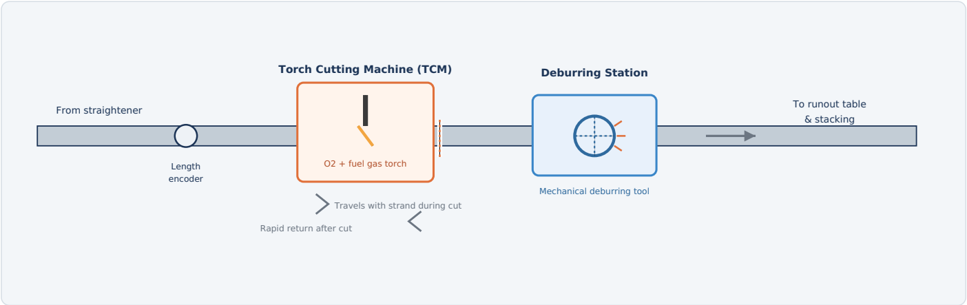
Fig. 6 — The TCM's torch carriage travels with the strand during each cut, then returns rapidly for the next one; a deburring station immediately downstream removes the resulting burr — by grinding, milling, or another mechanical method — before the piece moves on.
