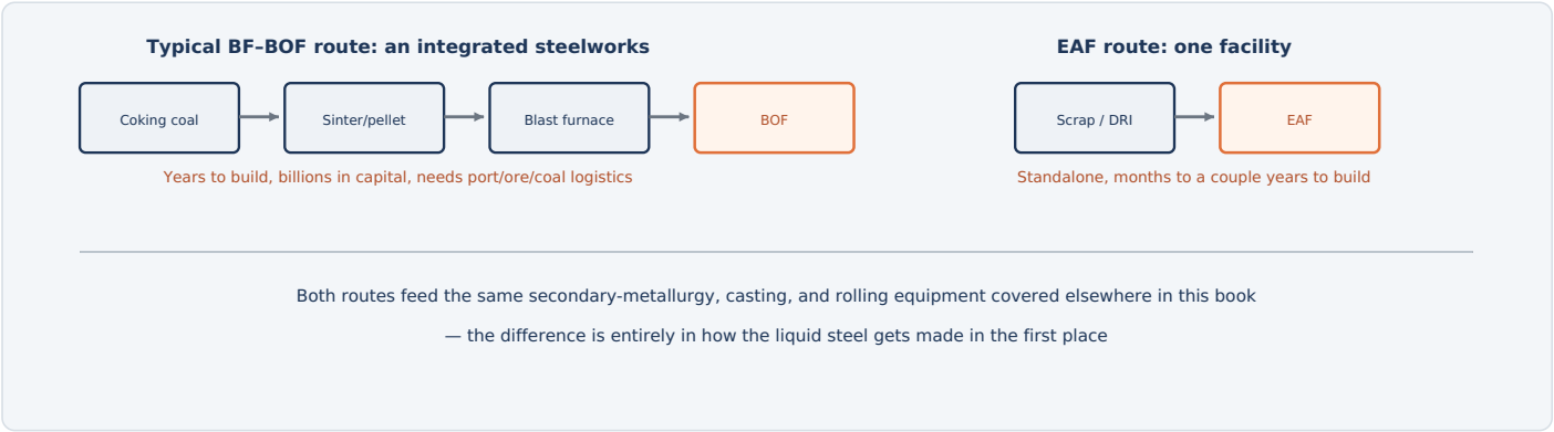
Fig. 5 — A BOF is most commonly tied to an entire integrated steelworks upstream of it, though smelting-reduction routes are a proven exception; an EAF is a complete melting solution on its own, which explains much of the structural cost advantage driving new investment decisions.
