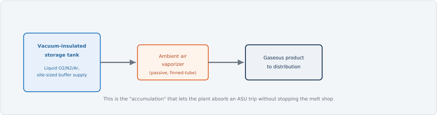
Fig. 4 — Liquid storage tanks hold a site-sized buffer of supply, commonly on the order of days but determined by plant-specific reliability and logistics decisions; ambient air vaporizers convert liquid back to usable gas on demand, using surrounding heat rather than added energy.
