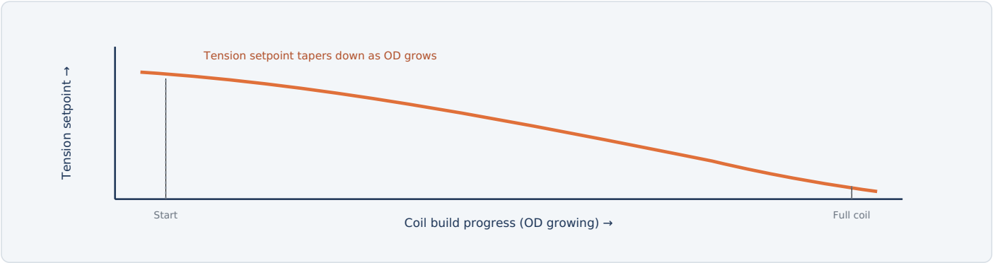
Fig. 3 — Rather than a fixed setpoint, tension is scheduled to fall as coil diameter grows, holding both mandrel torque and accumulated interlayer pressure within a safe band throughout the build.
