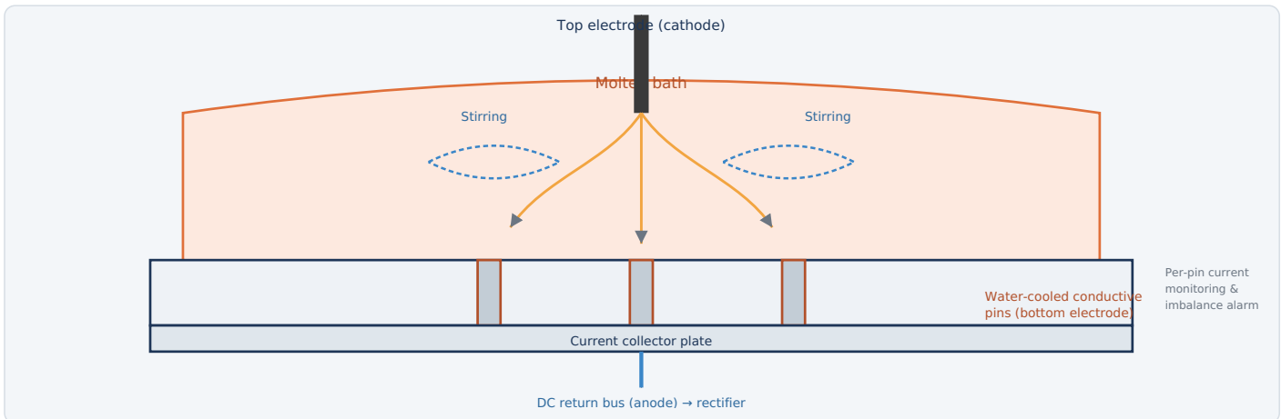
Fig. 4 — A pin-type bottom electrode (shown here) carries return current through the refractory bottom to a collector plate; fin-type and billet-type designs achieve the same function differently, with cooling method varying by OEM. Whichever design is used, the same vertical current flow through the bath produces a strong toroidal stirring pattern.
