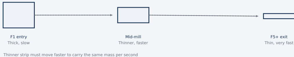
Fig. 1 — As thickness drops through the mill, speed rises to match, so the same tonnage per hour is always flowing past every point on the line simultaneously.
