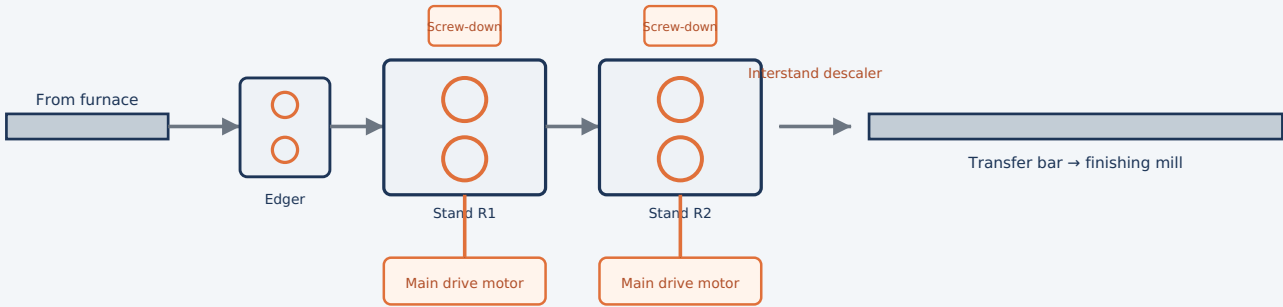
Fig. 2 — The roughing mill uses a series of reversing/tandem stands (with edgers) to reduce the slab's thickness in repeated passes, producing a long transfer bar.
