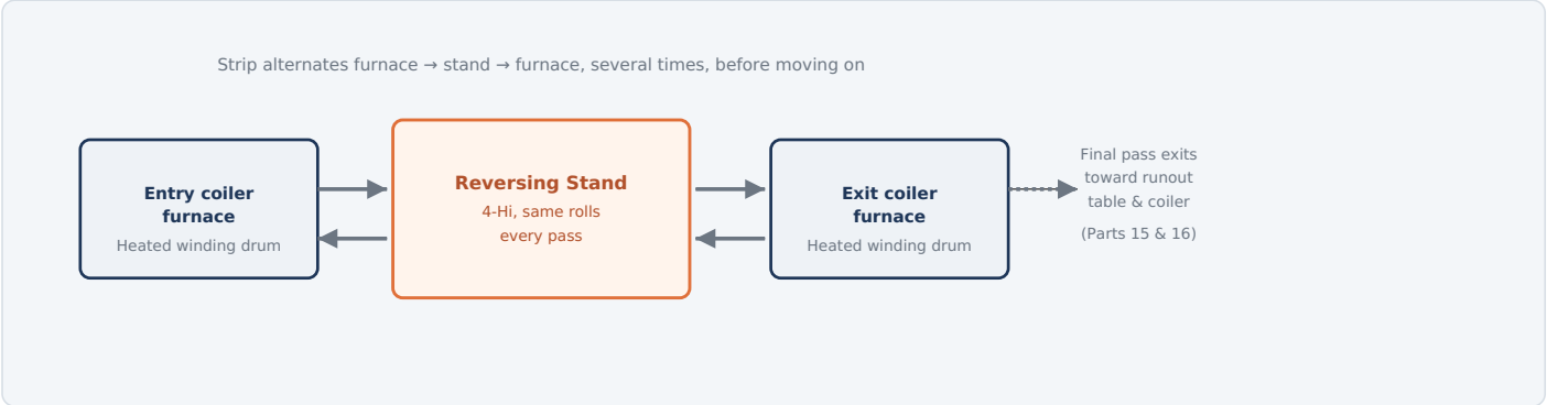
Fig. 1 — The transfer bar shuttles between the two coiler furnaces, taking one rolling pass through the single reversing stand each time it crosses, until the scheduled number of passes brings it to target gauge.
