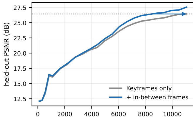
aria/aria1253 (7,321 it.) \Delta=+0.02 dB, -1,566 it. to match
