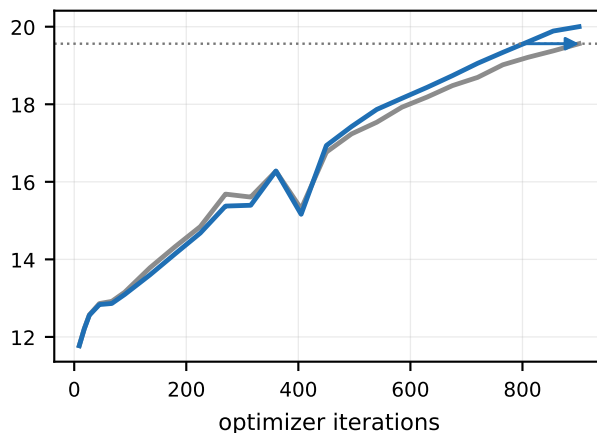
utmm/slow-straight-2 (901 it.) \Delta=+0.44 dB, -99 it. to match
