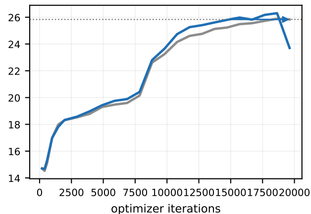
rpng/table_05 (19,621 it.) \Delta=-2.13 dB, -4,725 it. to match
