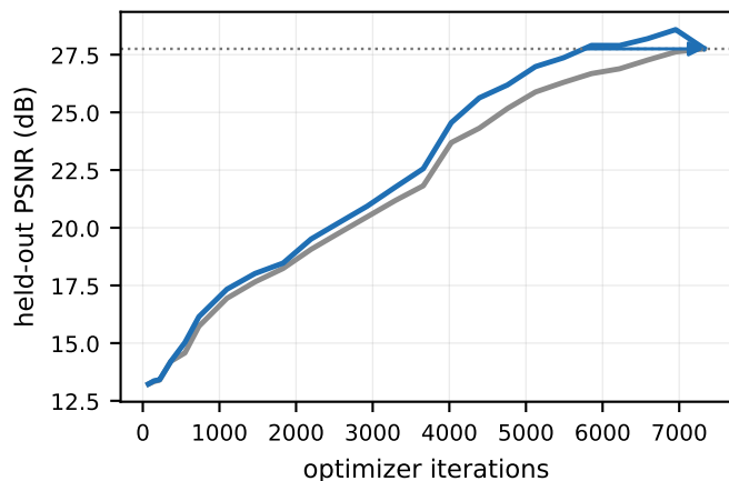
aria/aria1253 (7,321 it.) \Delta=+0.02 dB, -1,566 it. to match
