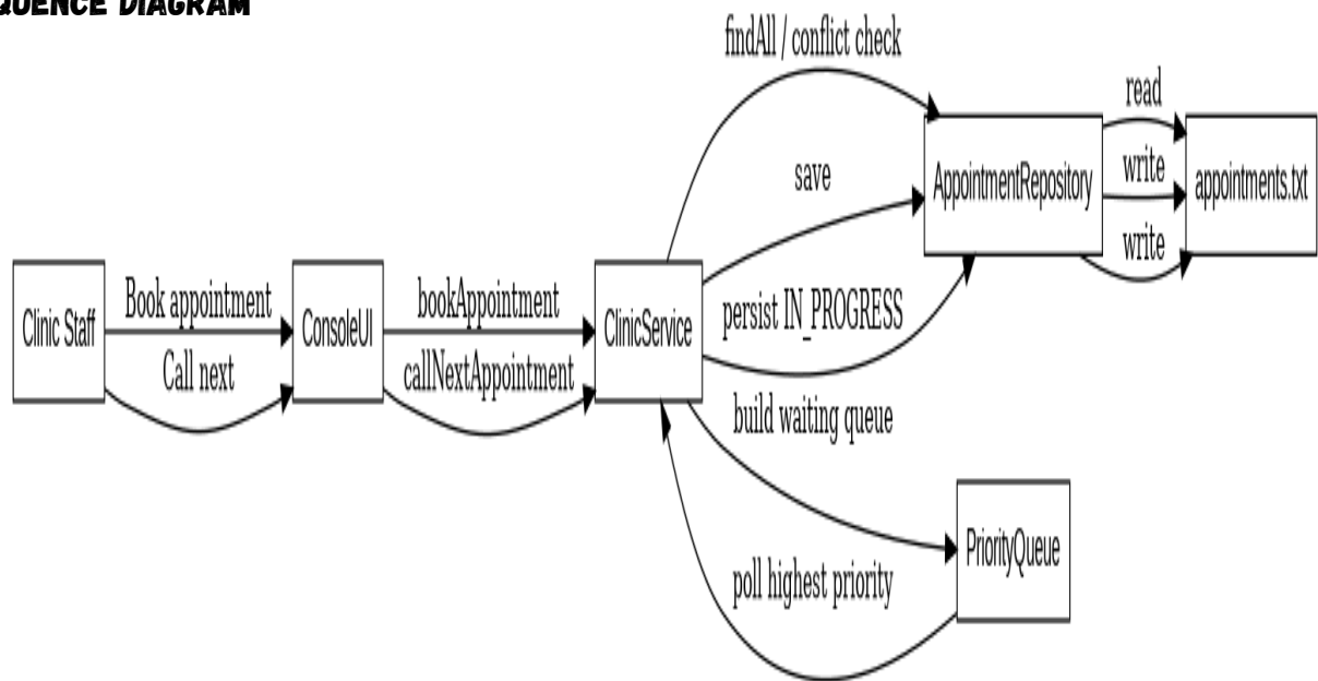
Figure 3. Appointment booking and queue-processing interaction.
