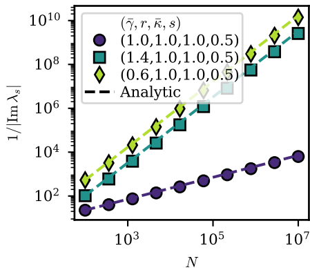
Exceptional point
