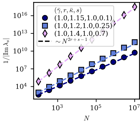
Regime B
