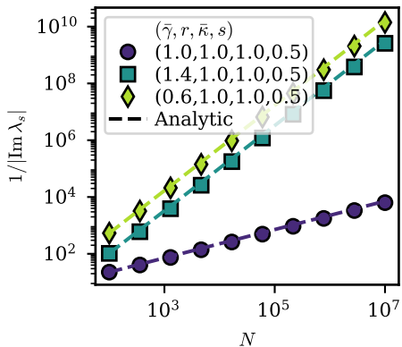
Exceptional point
