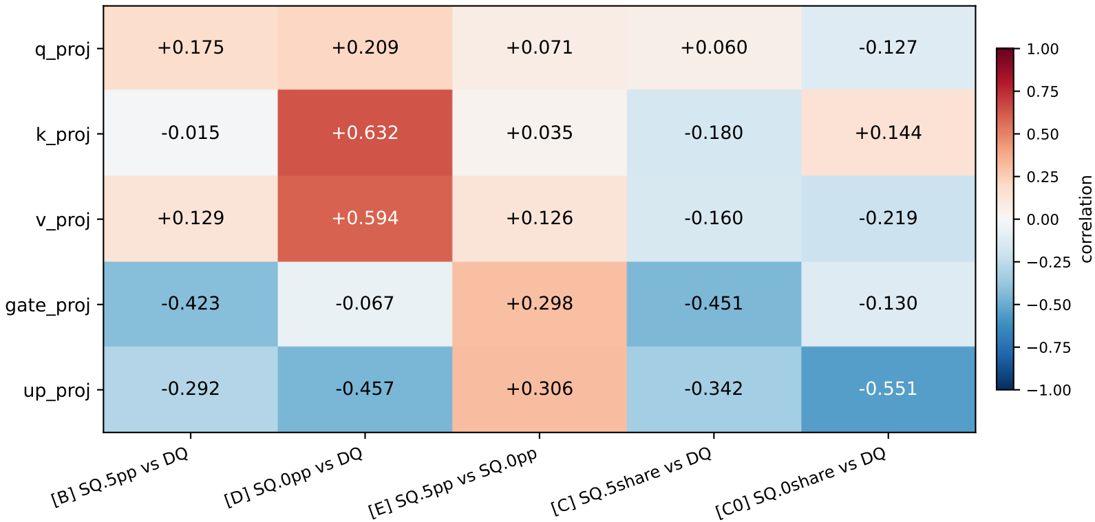
Qwen_Qwen2.5-7B — Pearson (mean over 28 layers)
