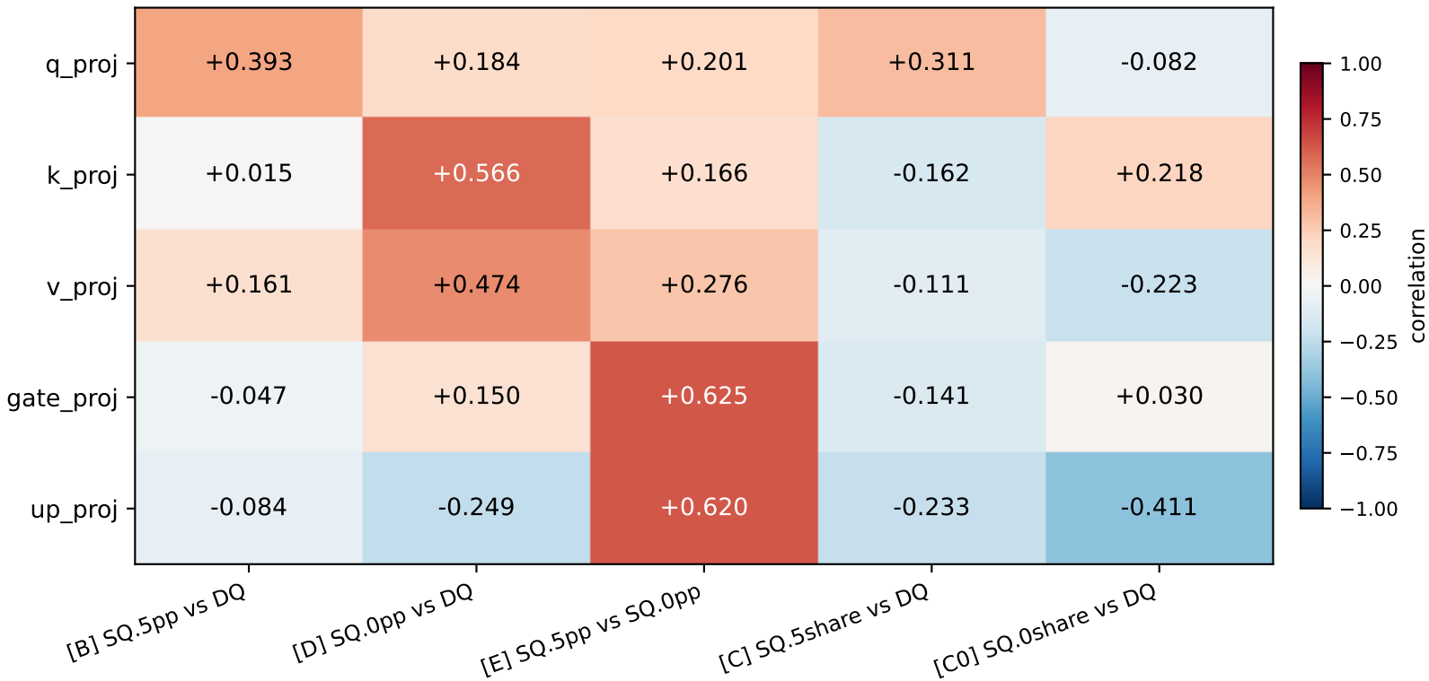
Qwen_Qwen2.5-7B — Spearman (mean over 28 layers)
