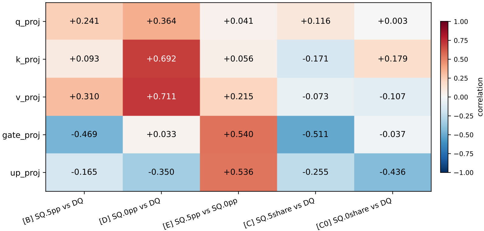
Qwen_Qwen2.5-7B — Log-Pearson (mean over 28 layers)
