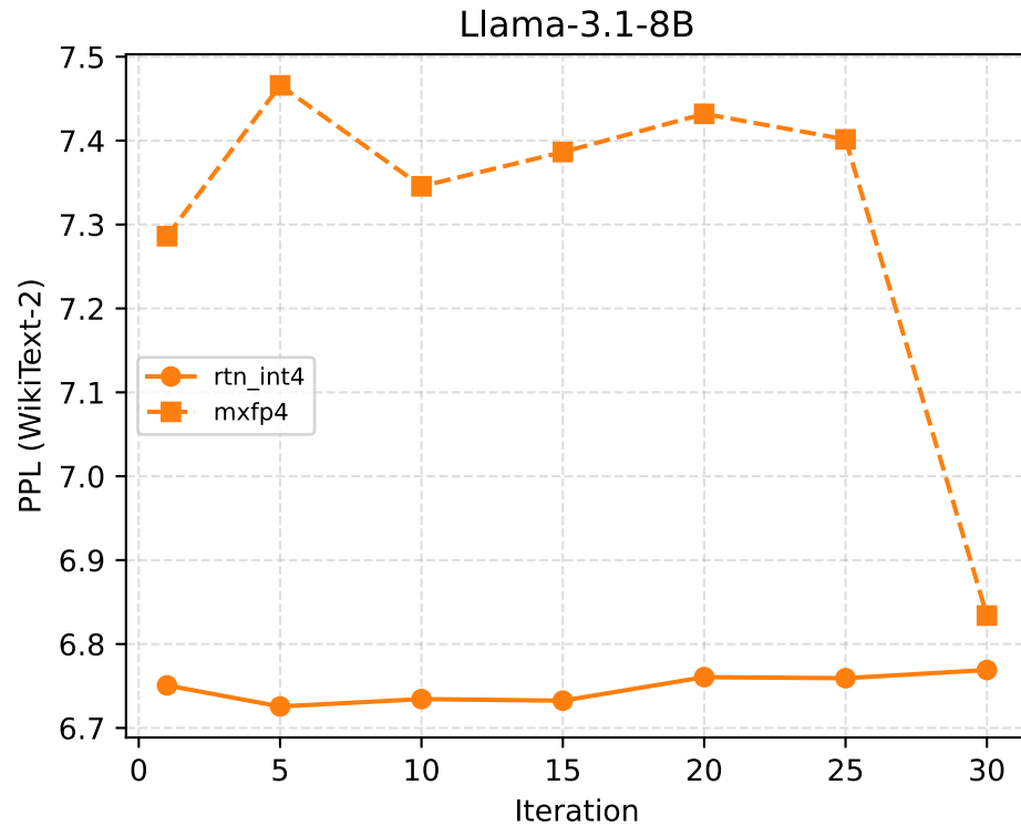
DualQuant: PPL vs Iteration
