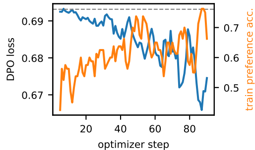
(a) Standard DPO training (5-step mean)
