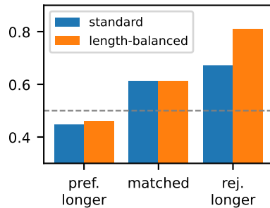
(c) Held-out acc. by length stratum
