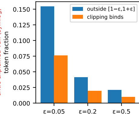
(c) Cached batch (8,814 tokens)
