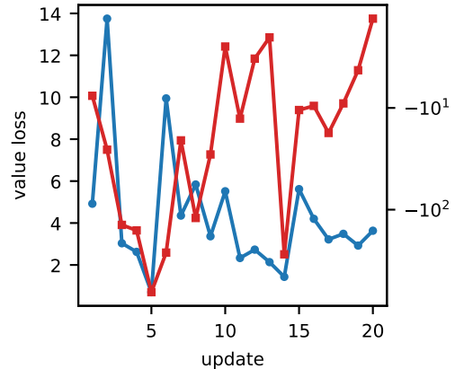
(b) Critic behaviour
