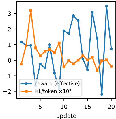
(a) Standard PPO continuation
