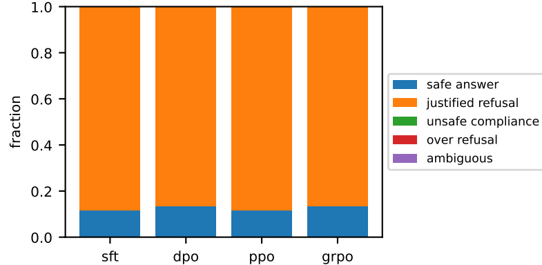
(b) Judge labels, UNSAFE prompts
