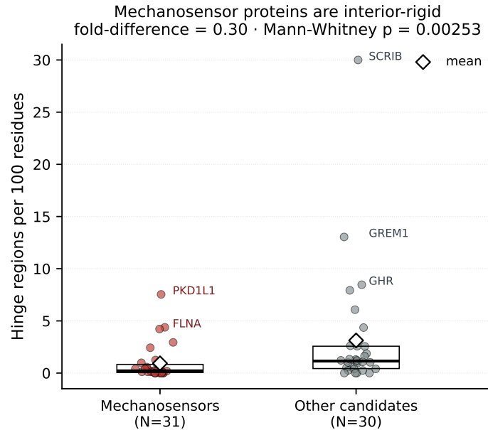
Figure 4: Mechanosensor proteins are interior-rigid. Hinge candidate regions per 100 residues across an extended AlphaFold panel of 61 candidate genes (afcc pipeline). Mechanosensors (Mechanotransduction/Proprioception/Cilia pathway tags, N = 31 ) have \sim 70\% fewer hinges per residue than other candidate proteins ( N = 30 ): mean 0.93 vs 3.12, fold-difference 0.30, Mann-Whitney p = 0.003 . Box: interquartile range; horizontal bar: median; diamond: mean. This rigid-interior signature is consistent with mechanosensors operating as cooperative rigid-body conformational switches rather than flexible-jointed sensors — a structural correlate of the anisotropy gap shown in Figure 3.
