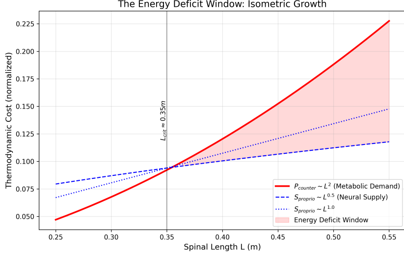
Figure 6: Thermodynamic Collapse: The Energy Deficit Window. (A) The metabolic power P_{\text{counter}} (red) required to maintain the Counter-Curvature active standing wave scales with spinal length as L^2 (assuming isometric growth) or L^3 (volumetric tone). (B) In contrast, the nutrient supply capacity of the avascular intervertebral disc (blue) scales sub-linearly ( L^{0.5} to L^1 ). The intersection at L_{\text{crit}} \approx 0.35 m marks the onset of the Energy Deficit Window ( L > L_{\text{crit}} ). Structural analysis of Thermodynamic Cost Proteins (Table 2) reveals the molecular basis of this deficit: high-anisotropy sensors like Piezo2 and Lamin A/C (demand-side) are structurally expensive to maintain [43], while compact supply-side enzymes (PLOD1, MMPs) are cheaper but rate-limited [44]. In the deficit regime, the system cannot afford the high-fidelity state, triggering a Convective Shutdown [8] and a collapse into the low-energy scoliotic mode.
