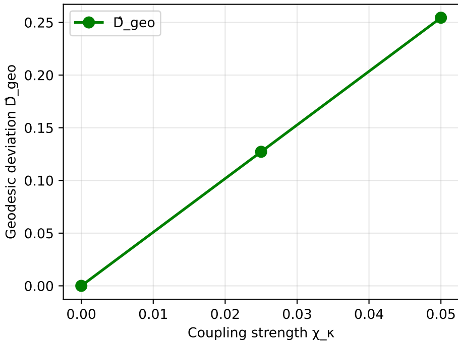
(C) Geodesic Deviation vs Coupling
