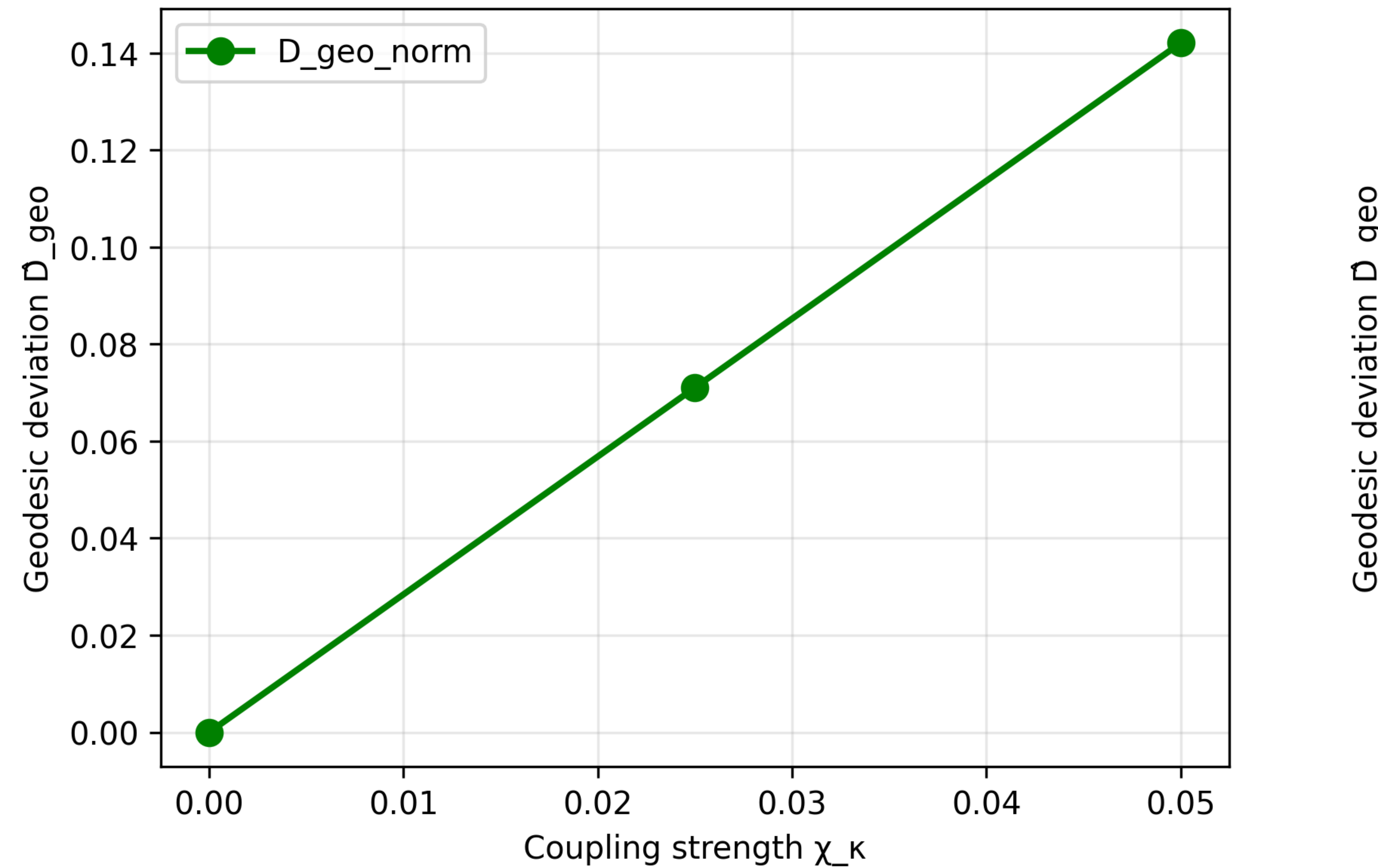
(C) Geodesic Deviation vs Coupling
