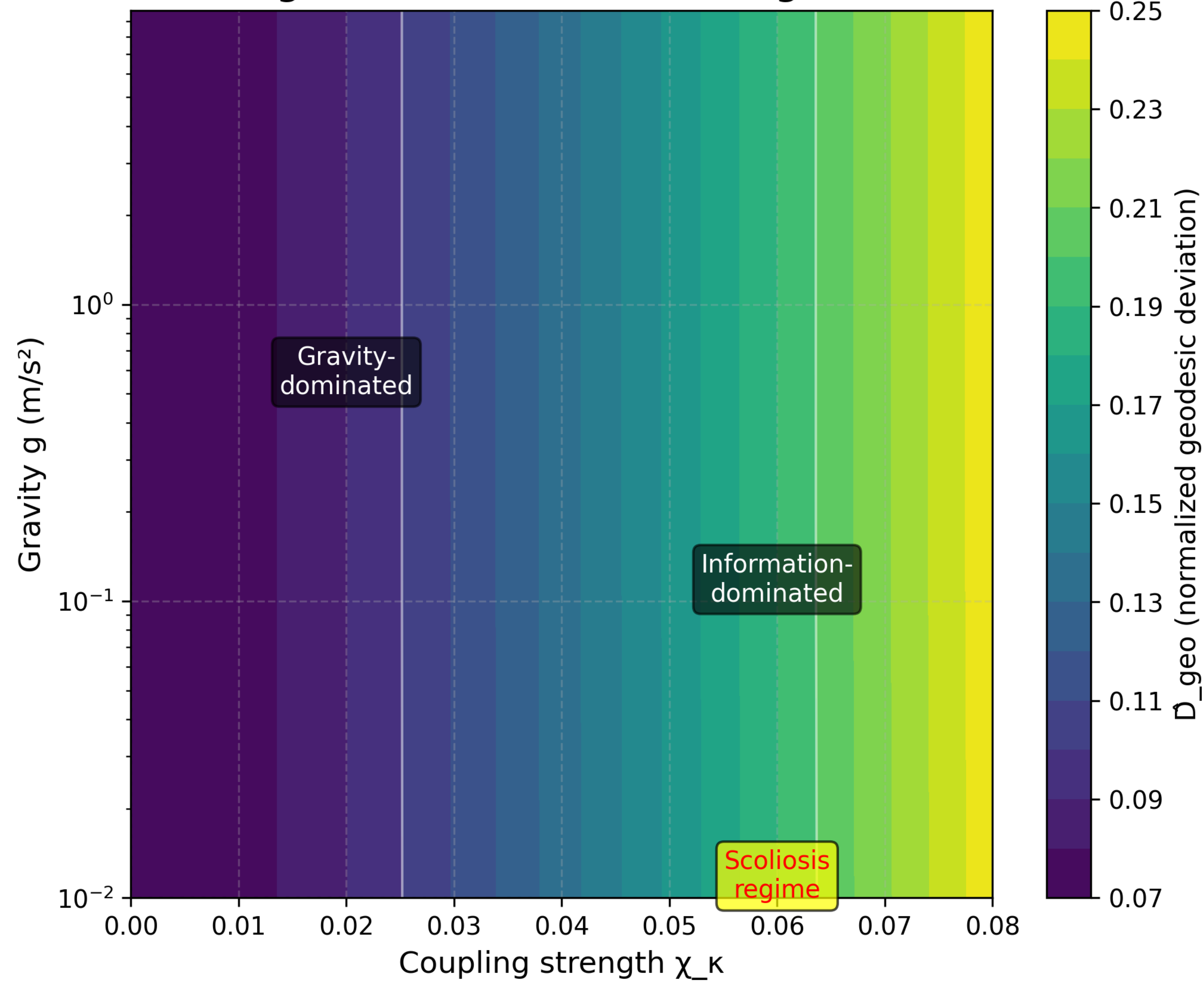
(A) Phase Diagram: Countercurvature Regimes + Scoliosis
