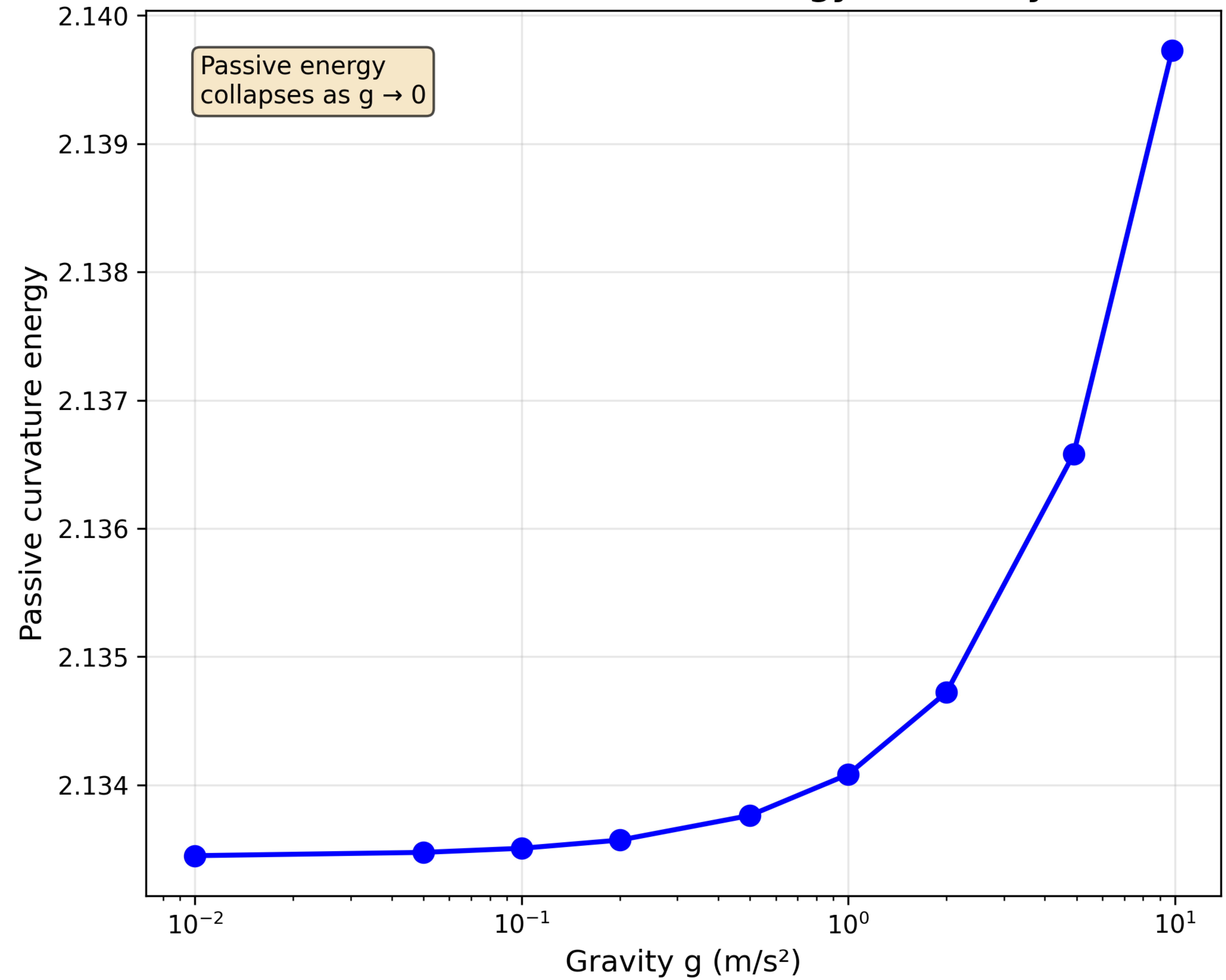
(B) Passive Curvature Energy vs Gravity
