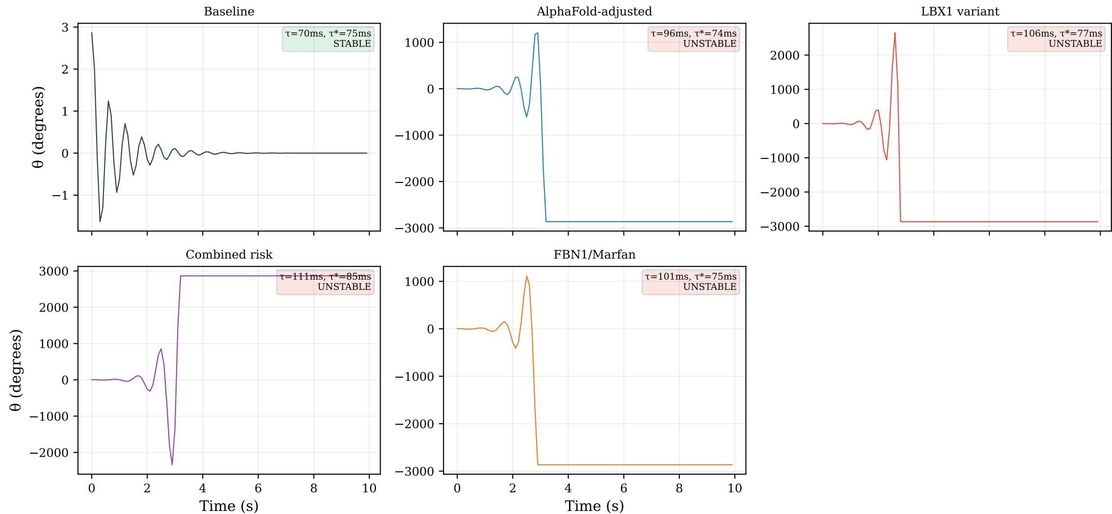
Figure 9: DDE Trajectories Under Molecular Parameterisation
