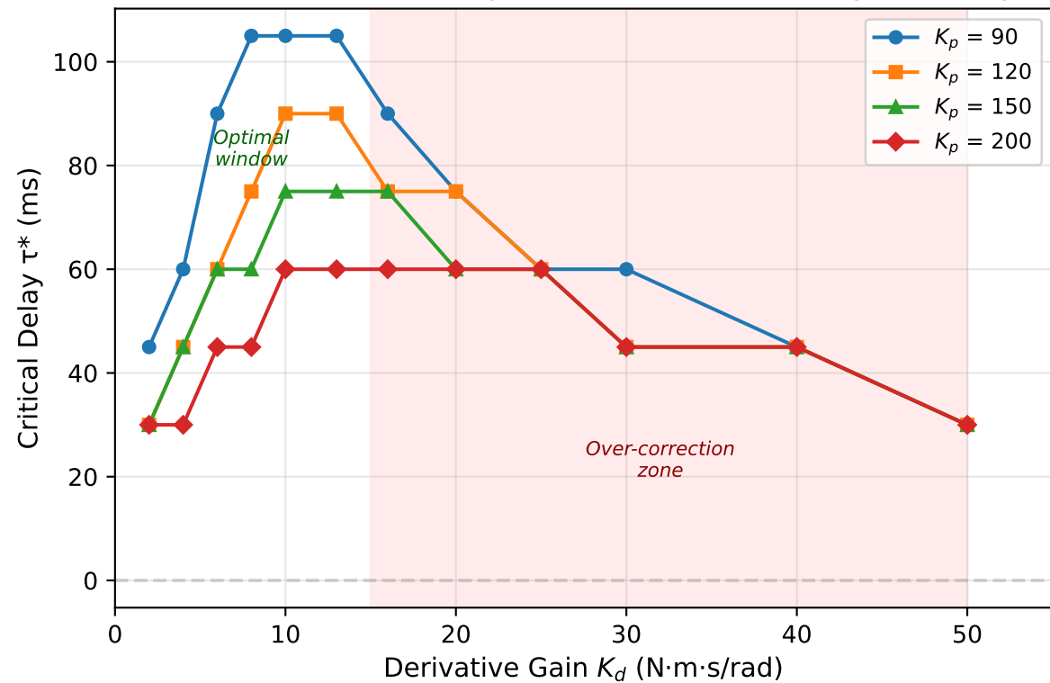
The Derivative Gain Trap: Non-Monotonic Stability Boundary
