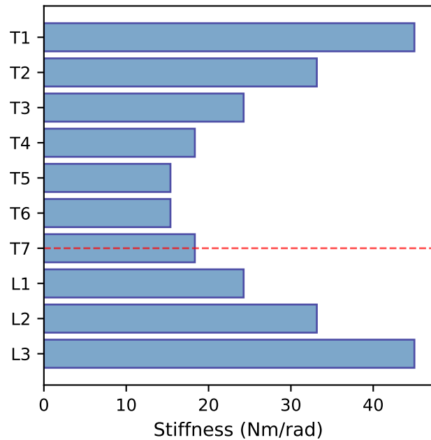
A. Segment Stiffness
