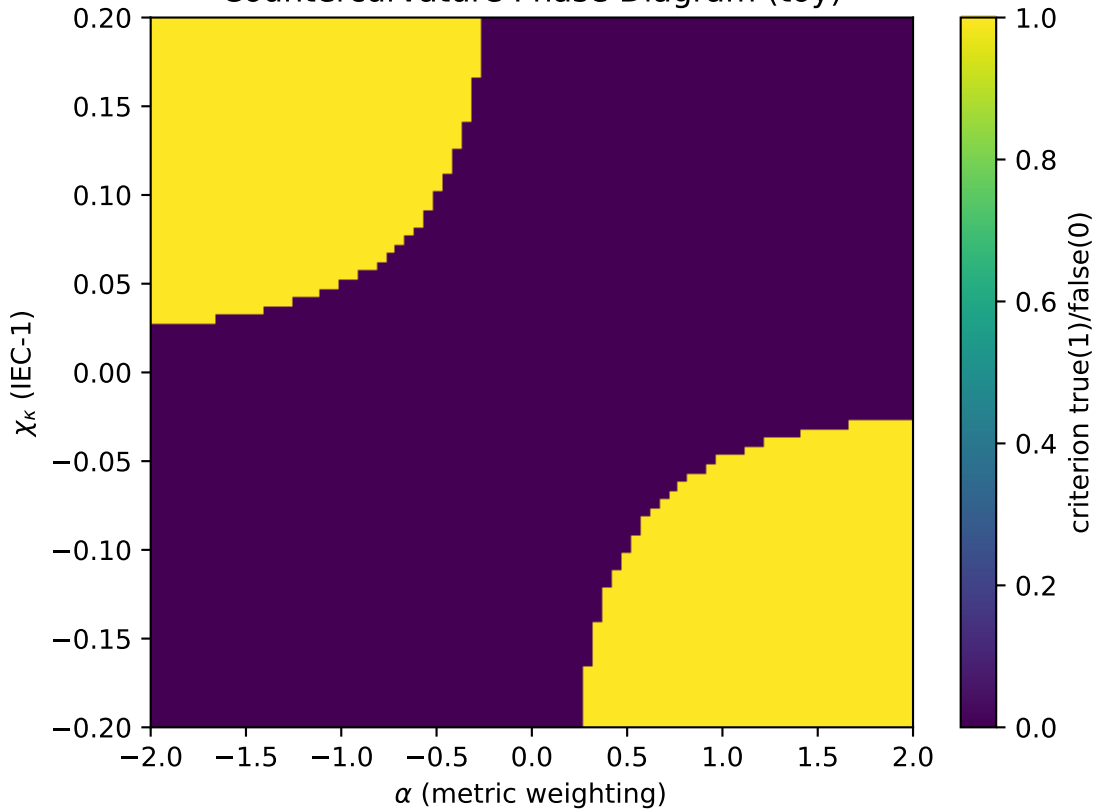
Countercurvature Phase Diagram (toy)
