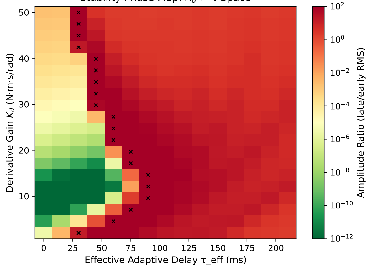
Stability Phase Map: K_d \times \tau Space
