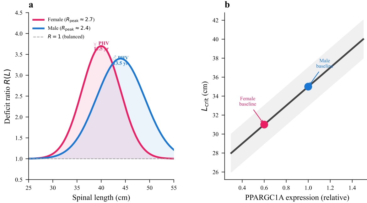
Fig. 4 | Sexual dimorphism in the Energy Deficit Window. a , Female (red) and male (blue) deficit ratio profiles. Girls show a narrower but deeper window ( R_{\text{peak}} = 2.7 vs. 2.4). b , Sensitivity of L_{\text{crit}} to PPARGC1A expression level, showing that lower female basal expression shifts vulnerability to shorter spinal lengths.
