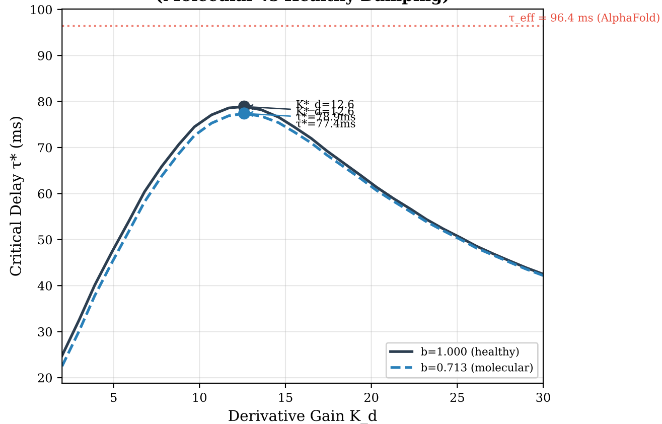
Figure 8: The Derivative Gain Trap (Molecular vs Healthy Damping)
