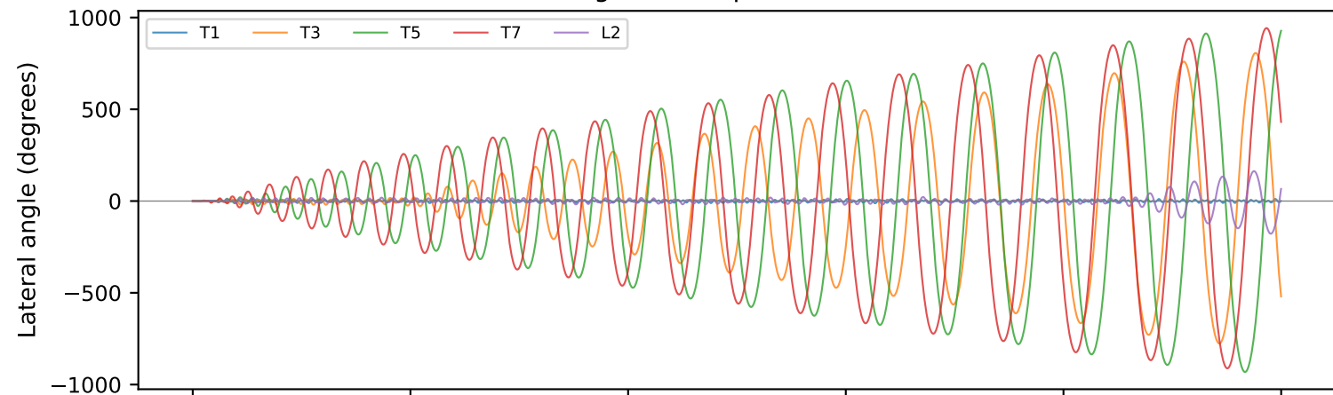
B. Coupled Axial Rotation
