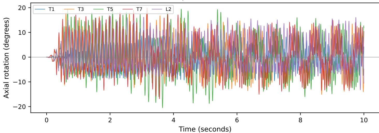
B. Coupled Axial Rotation
