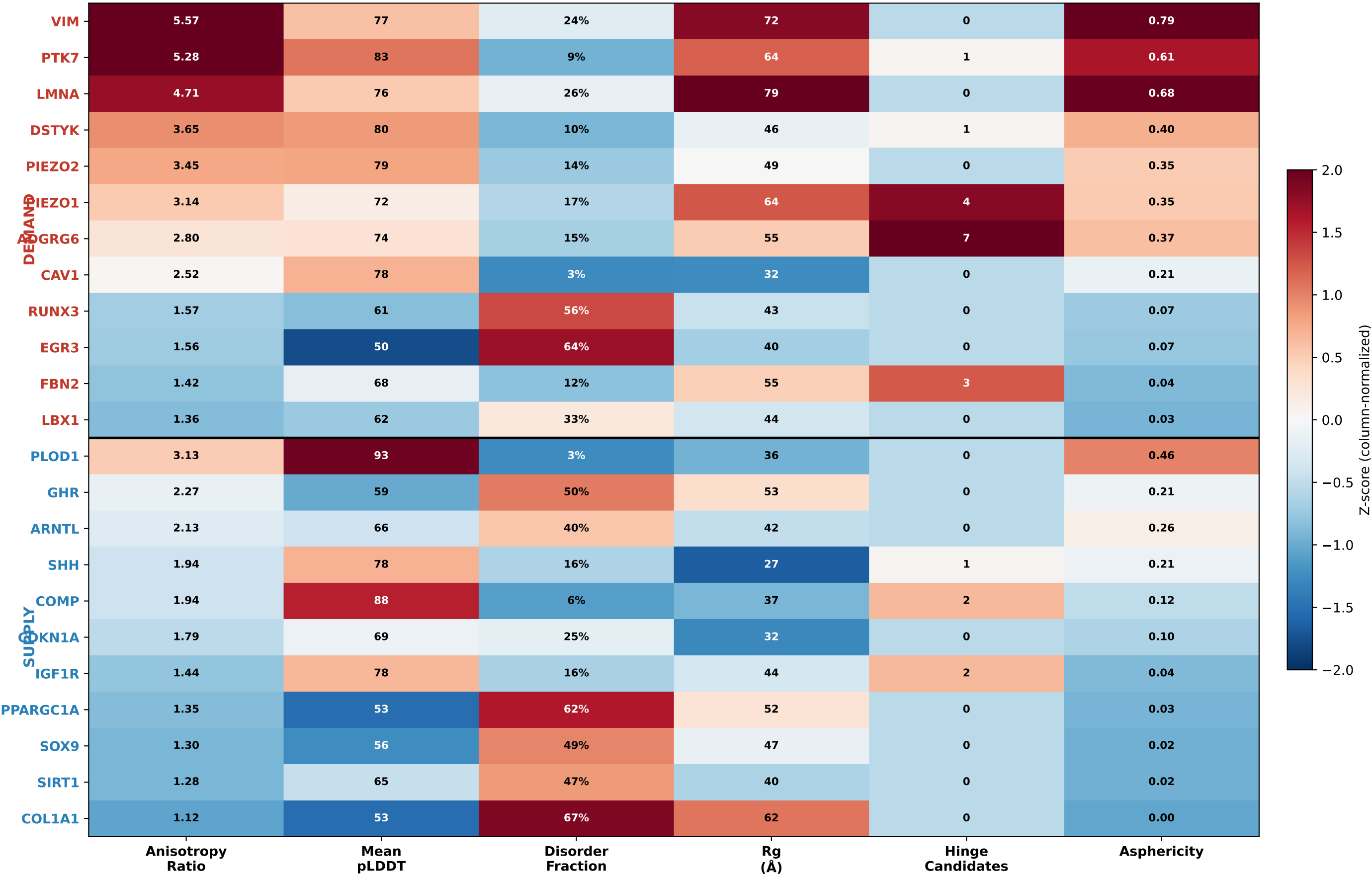
AlphaFold Structural Metrics Heatmap — 23 IEC Framework Proteins (Red = high relative value, Blue = low relative value)
