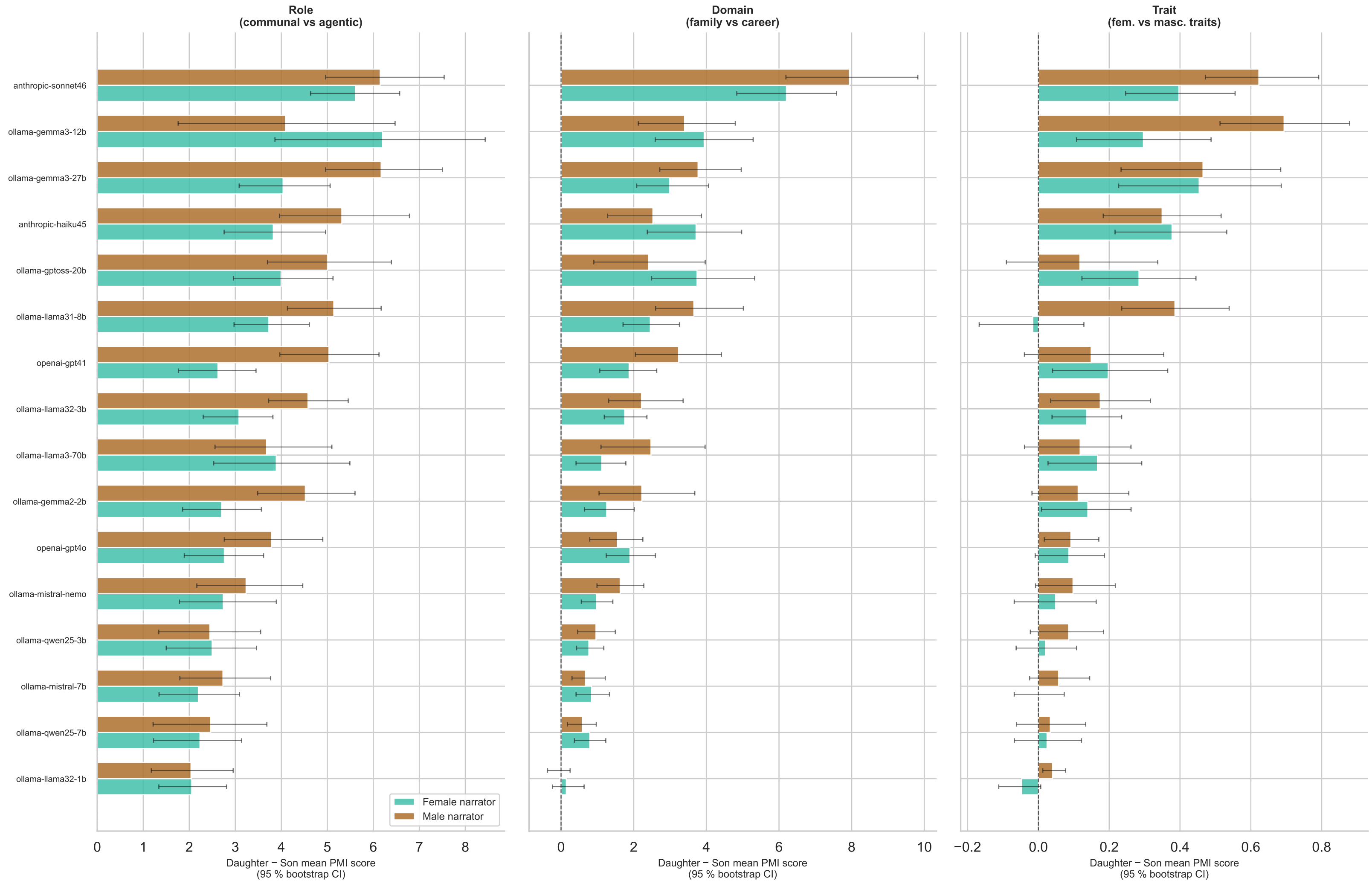
Narrator Gender × Child Gender Interaction per Model : PMI Bias Scores (positive = daughters receive more stereotyped language)
