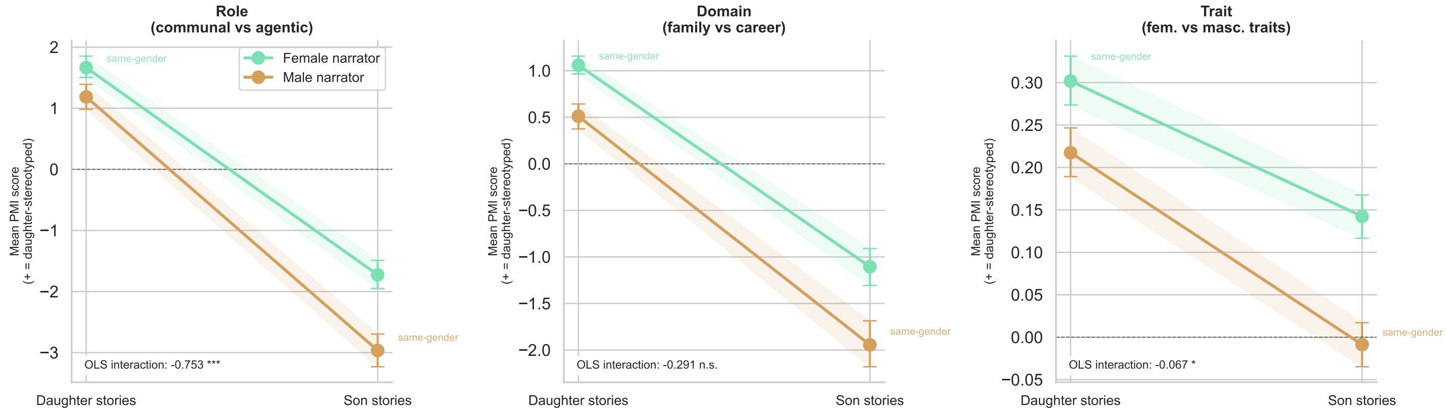
Narrator Gender × Child Gender Interaction : PMI Bias Scores (All Models) Parallel lines = no moderation; steeper line = narrator role amplifies bias (shading = 95 % bootstrap CI)
