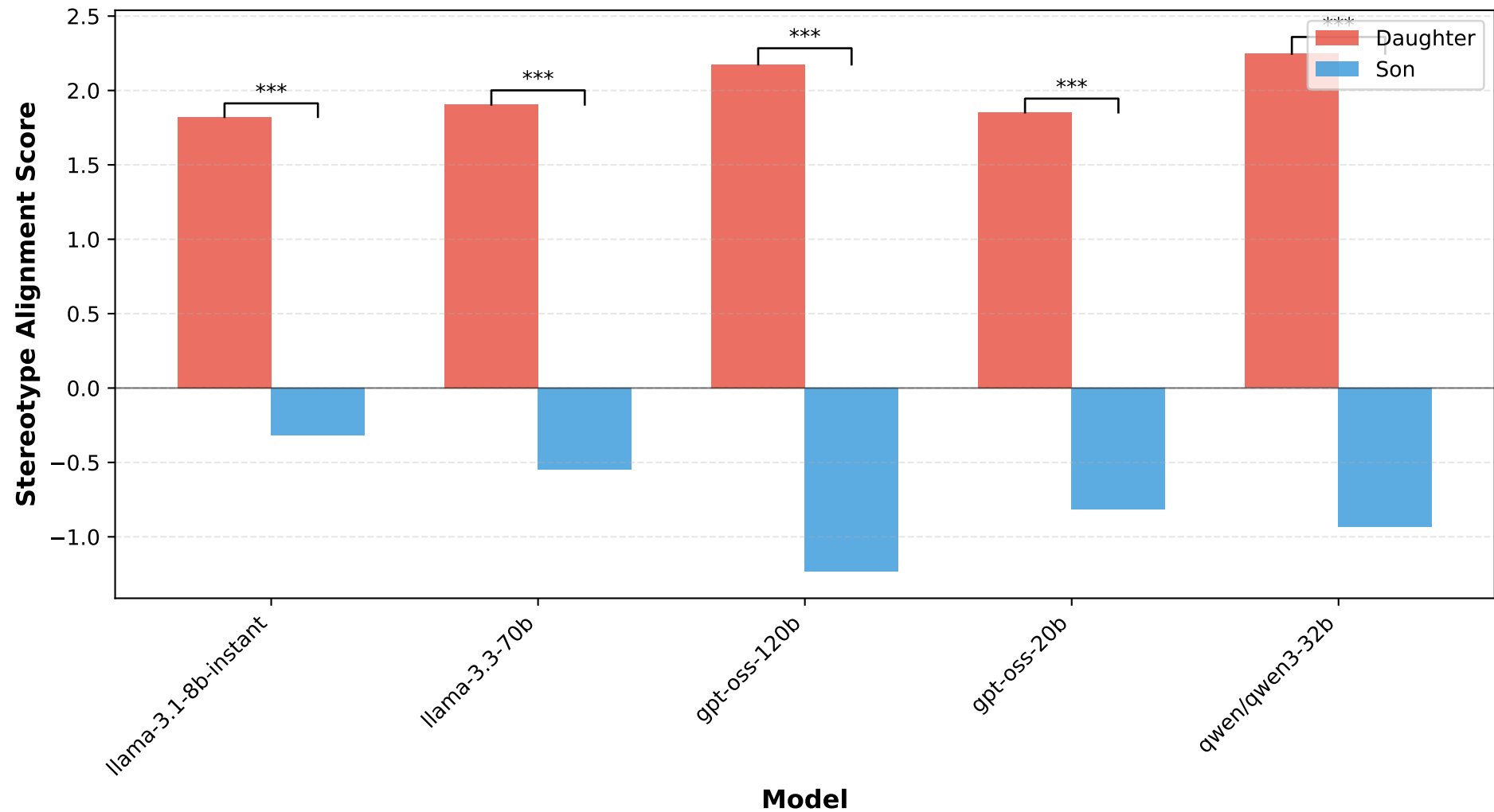
Stereotype Alignment Score by Model and Child Gender
