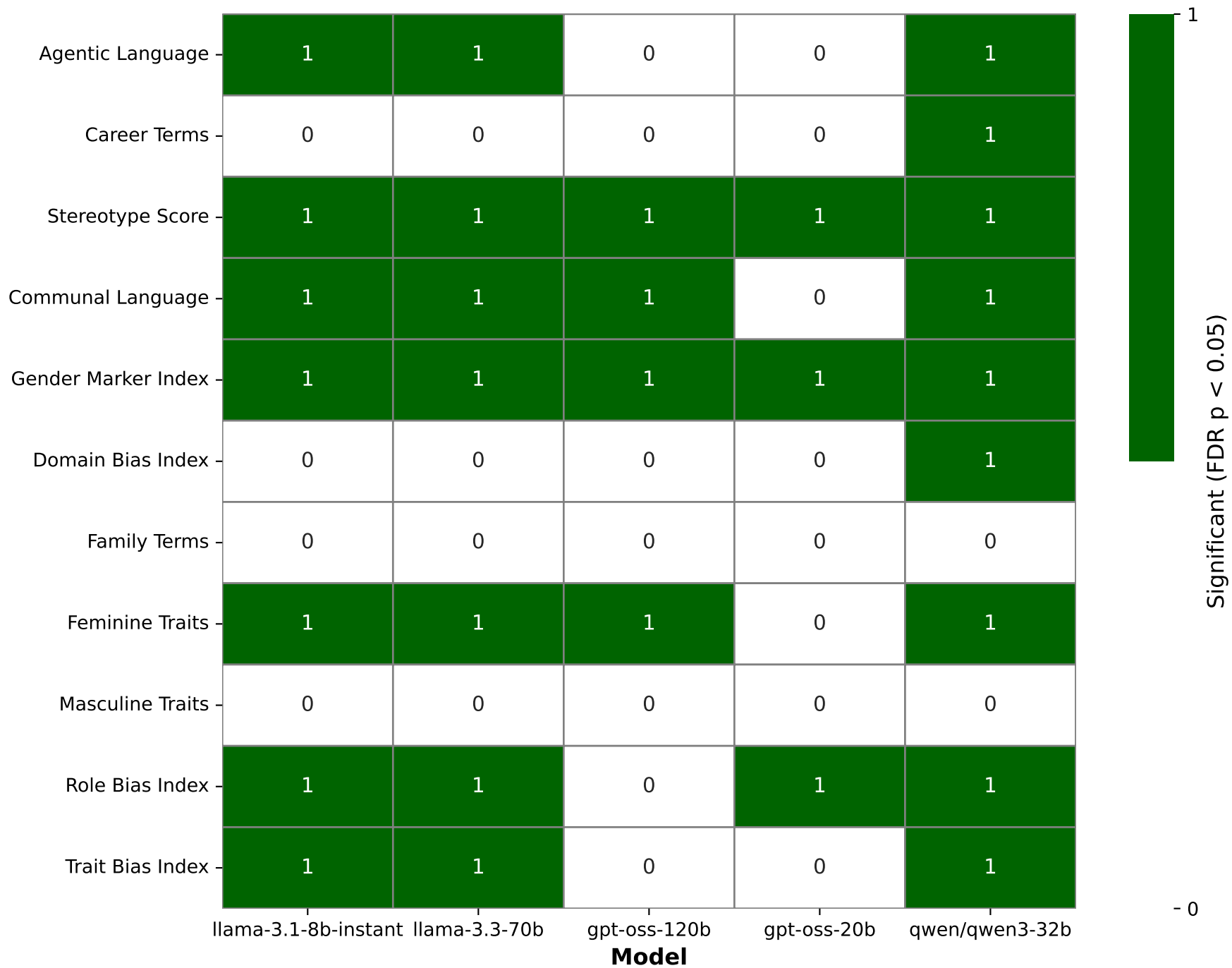
Statistical Significance by Model and Metric (FDR-corrected p < 0.05 )
