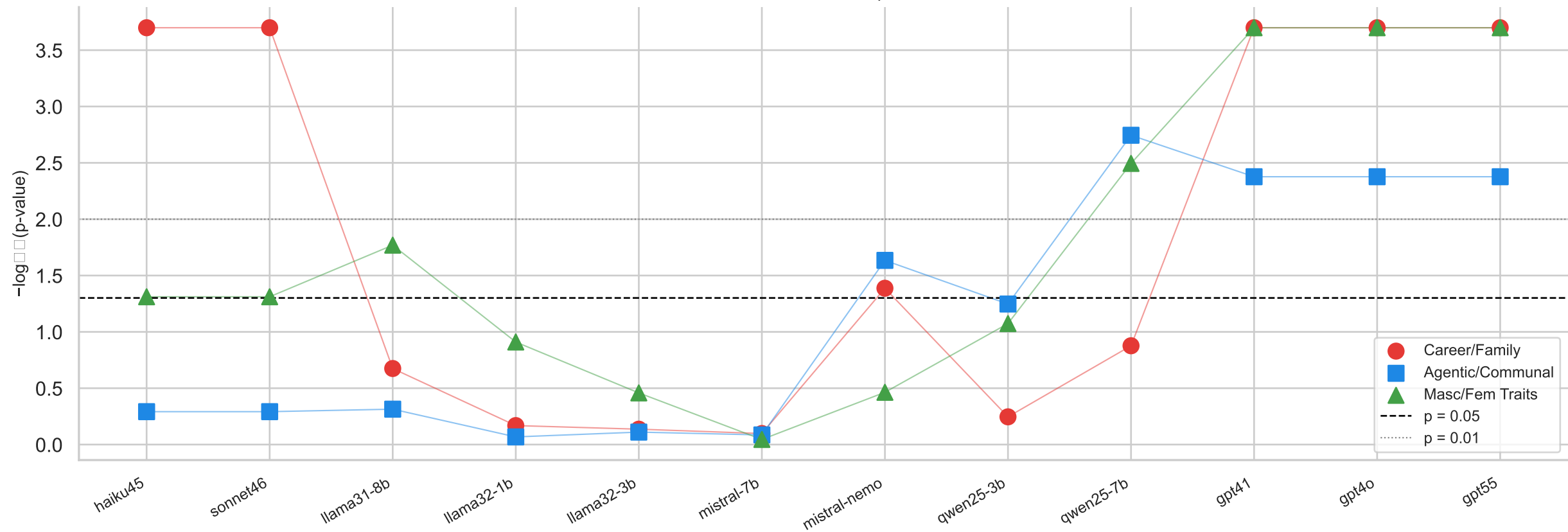
WEAT Statistical Significance (final layer, one-tailed permutation test)
