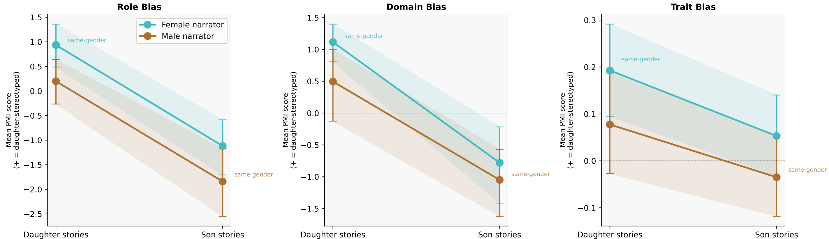
Narrator Gender × Child Gender Interaction — gemma2-2b PMI Bias Scores · Parallel lines = no moderation · Steeper / crossing lines = narrator amplifies bias (shading = 95 % bootstrap CI)
