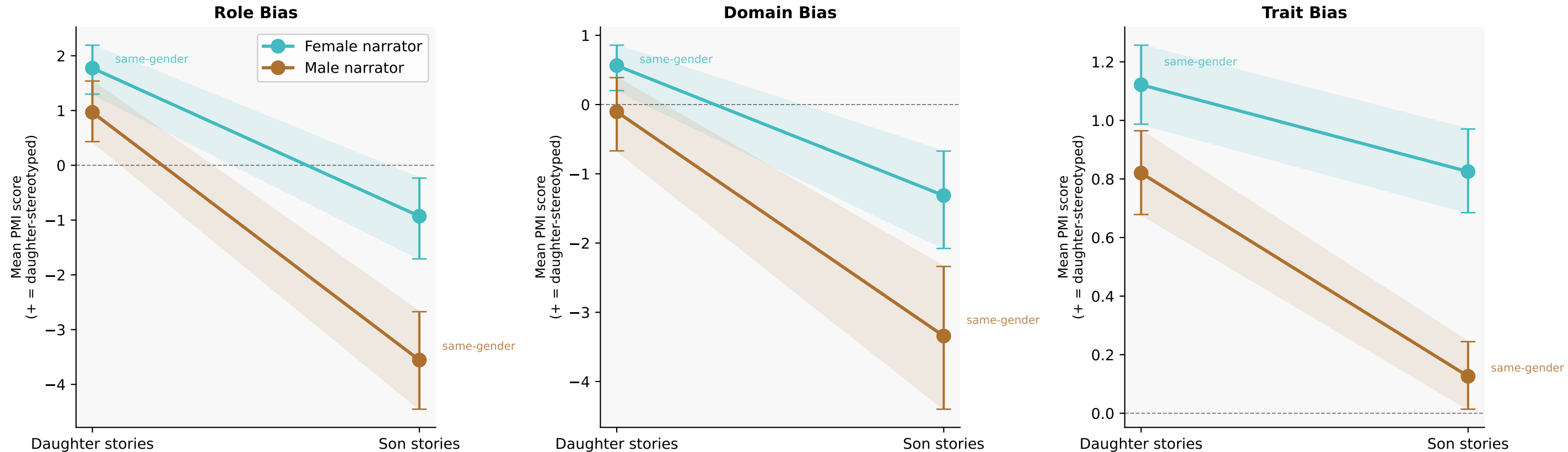
Narrator Gender × Child Gender Interaction — gemma3-12b PMI Bias Scores · Parallel lines = no moderation · Steeper / crossing lines = narrator amplifies bias (shading = 95 % bootstrap CI)
