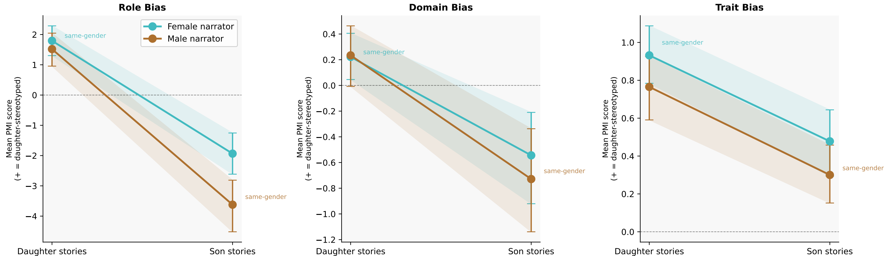
Narrator Gender × Child Gender Interaction — gemma3-27b PMI Bias Scores · Parallel lines = no moderation · Steeper / crossing lines = narrator amplifies bias (shading = 95 % bootstrap CI)
