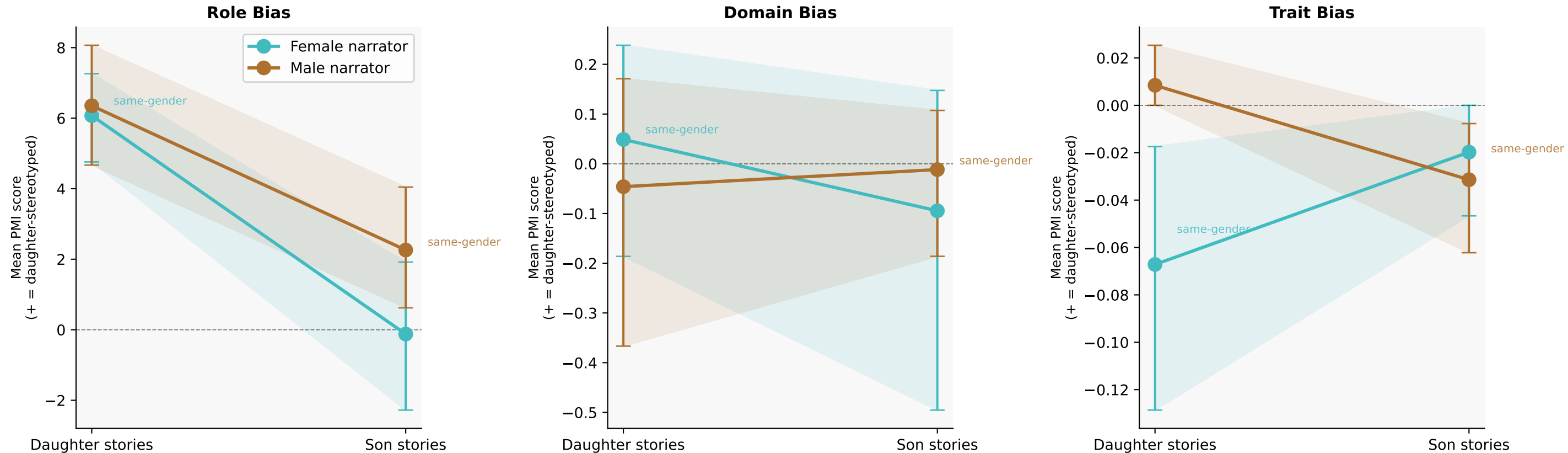
Narrator Gender × Child Gender Interaction — llama32-1b PMI Bias Scores · Parallel lines = no moderation · Steeper / crossing lines = narrator amplifies bias (shading = 95 % bootstrap CI)
